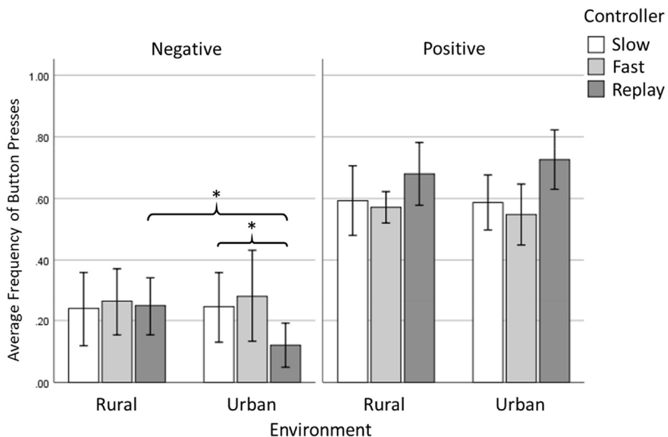
Fig. 6. Average positive and negative button presses for each controller in the Rural and Urban environment (* p < 0.05 ). Error bars represent \pm 1 standard error.
