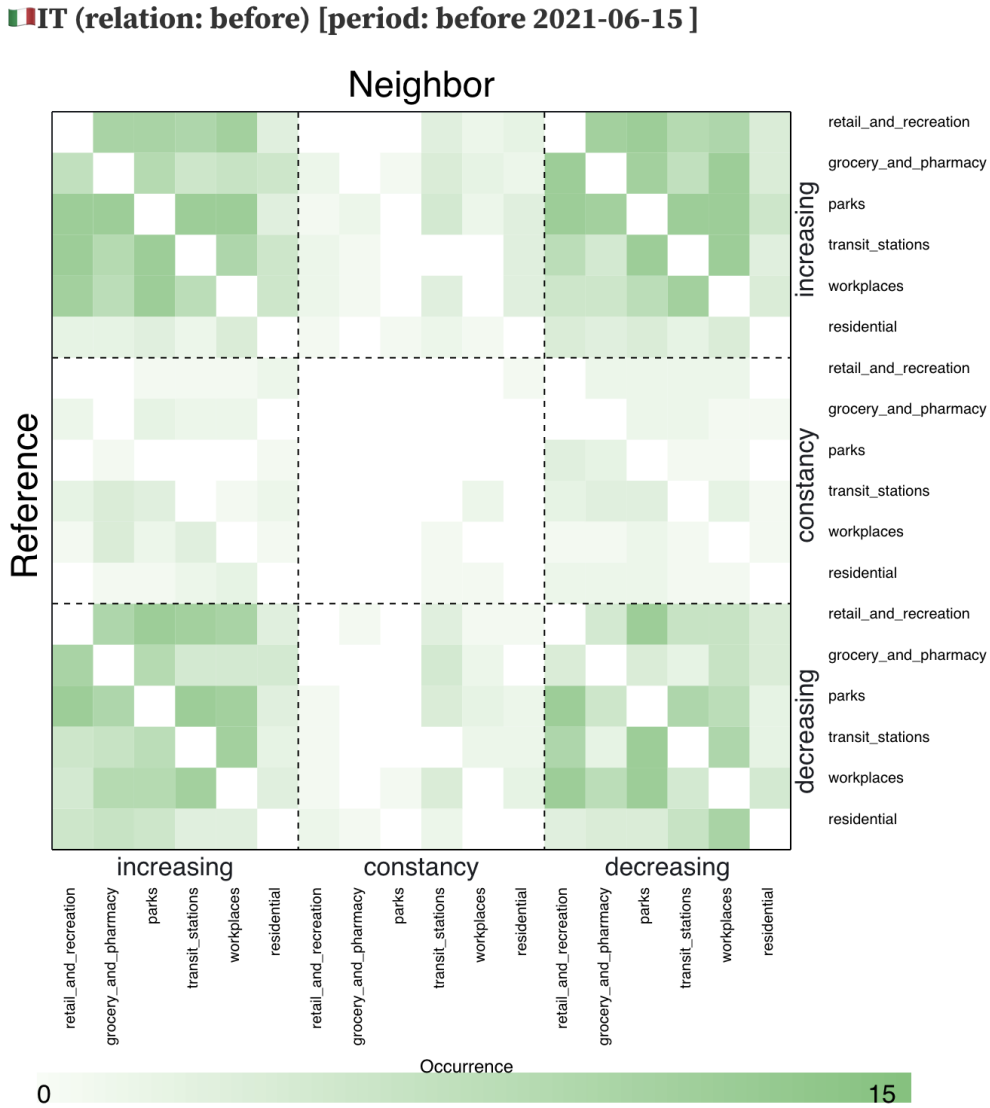
Figure 7: Relation occurrences matrix: Each cell represents the frequency of the target relation (before in this example) between two patterns across various attributes. The matrix rows and columns are divided into three blocks corresponding to increase, constancy, and decrease patterns. Darker shades indicate more frequent occurrences, while lighter ones signify fewer.
