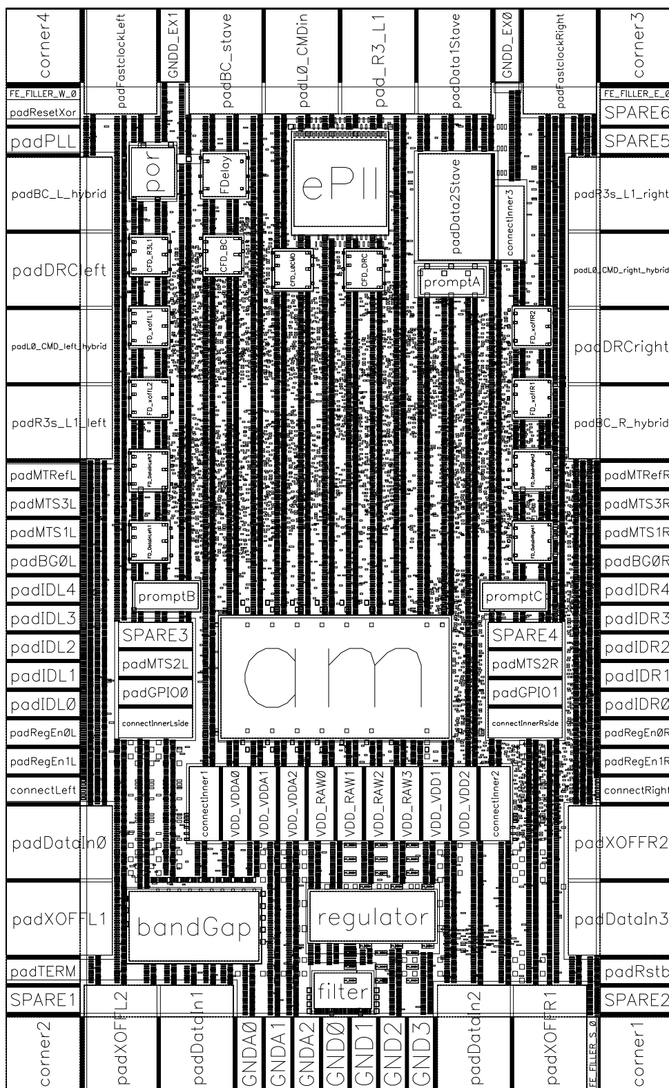
Figure 11. HCC130 Pad Ring and floorplan.
