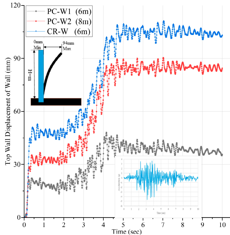
Figure 6. Top Displacement of Wall.
