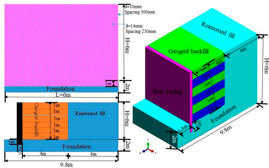
Figure 2. Detailed dimensions of reinforcement concrete MSE wall structural components.
