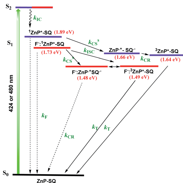
Fig. 4 Energy level diagram depicting excited state charge separation and recombination upon Soret band excitation in ZnP-SQ (purple) and \text{F}^- : ZnP-SQ (red). Abbreviations: F = fluorescence, IC = internal conversion, ISC = intersystem crossing, CS = charge separation, CR = charge recombination, S = singlet state and T = triplet state. Solid arrow = major path, dashed arrow = minor path.
