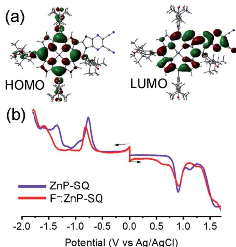
Fig. 3 (a) HOMO and LUMO structures of ZnP-SQ on B3LYP/6-31G* optimized structure. (b) DPV of ZnP-SQ (purple) and \text{F}^- : ZnP-SQ (red) in DCB containing 0.1 M (TBA) \text{ClO}_4 . Scan rate = 5 \text{ mV s}^{-1} , pulse width = 0.25 s, pulse height = 0.025 V.
