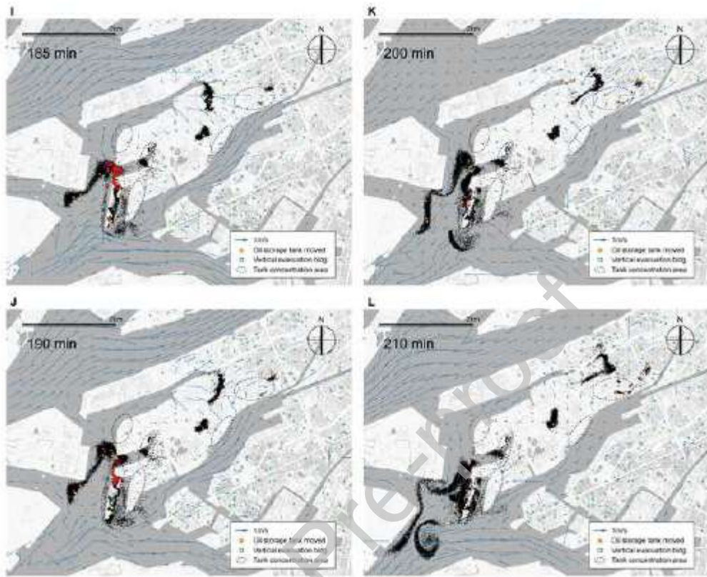
Figure 11. Examples of simulated tsunami-driven oil fire spreading (blue arrows represent tsunami flow velocity vectors; black and red particles represent unburned and burning oil particles, respectively).
