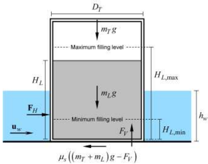
Figure 4. Schematic of a simplified model for oil storage tanks subjected to tsunami inundation flow.
