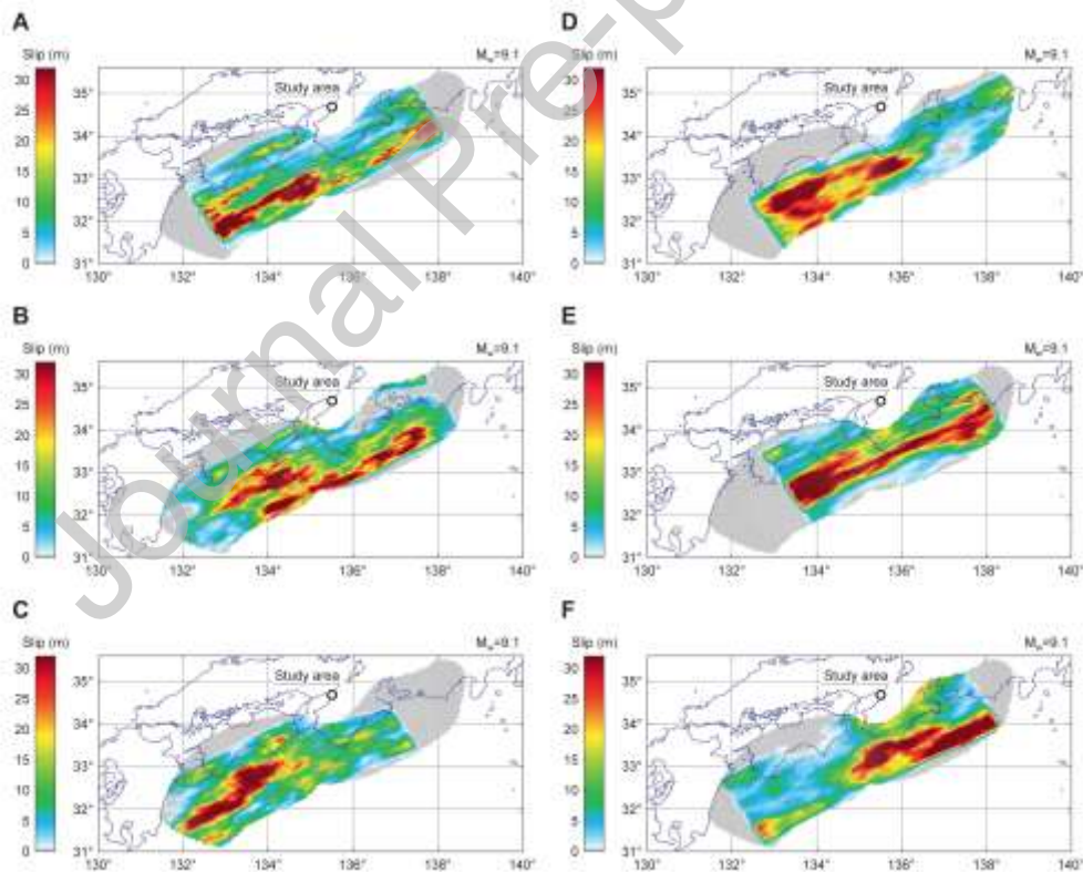
Figure 7. Examples of synthesized fault slip distributions for Mw 9.1 earthquakes in the Nankai Trough subduction zone.
