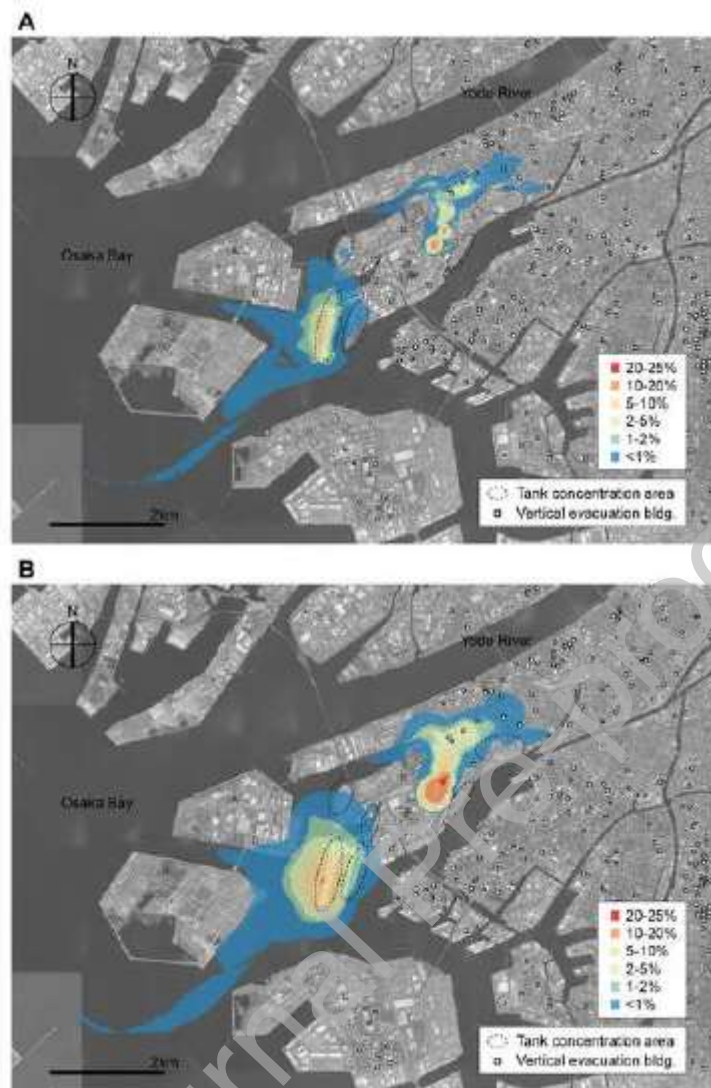
Figure 15. Probabilistic fire hazard maps obtained via 1040 tsunami-driven oil fire spread simulations: spatial distributions of the conditional exceedance probability of the maximum radiative heat flux with threshold values of (A) 10 kW/m 2 and (B) 2 kW/m 2 .
