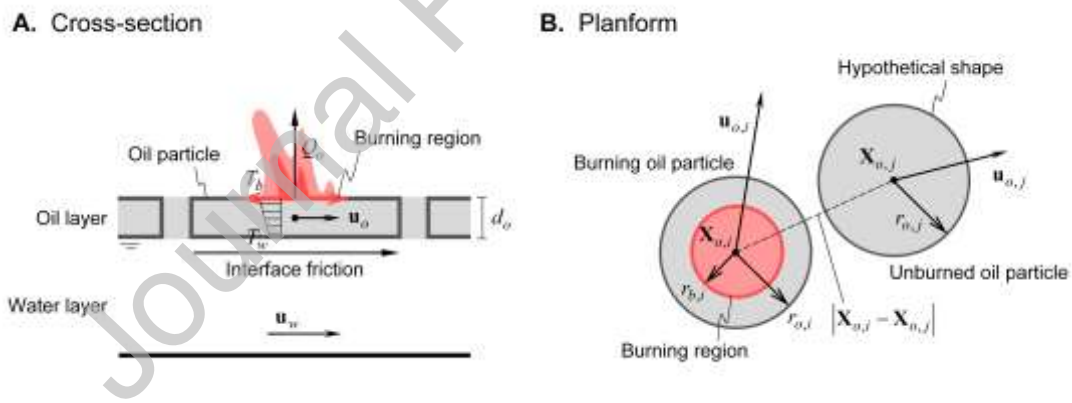
Figure 5. Schematic of a Lagrangian model for tsunami-driven oil fire spread [14].
