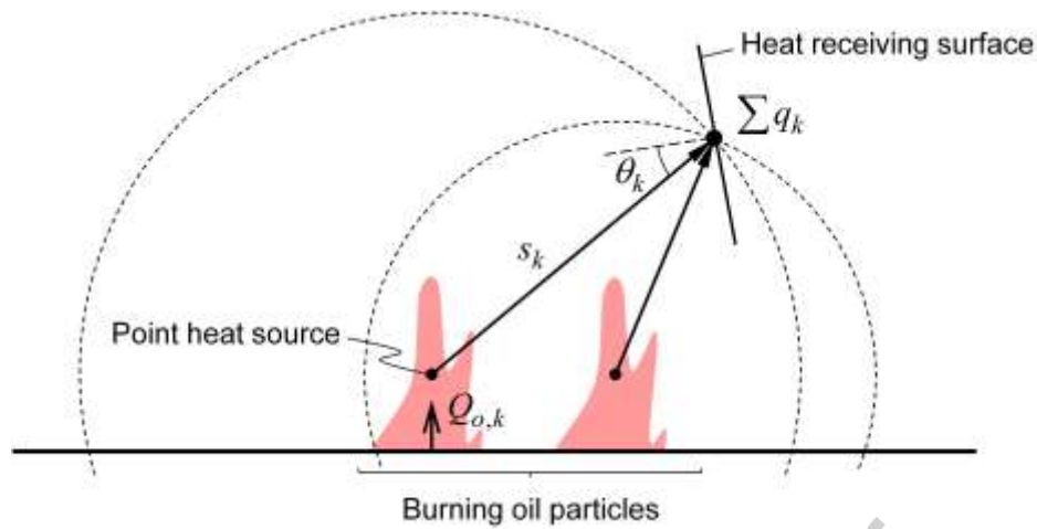
Figure 6. Schematic of a point source model for radiation heat transfer from flames.
