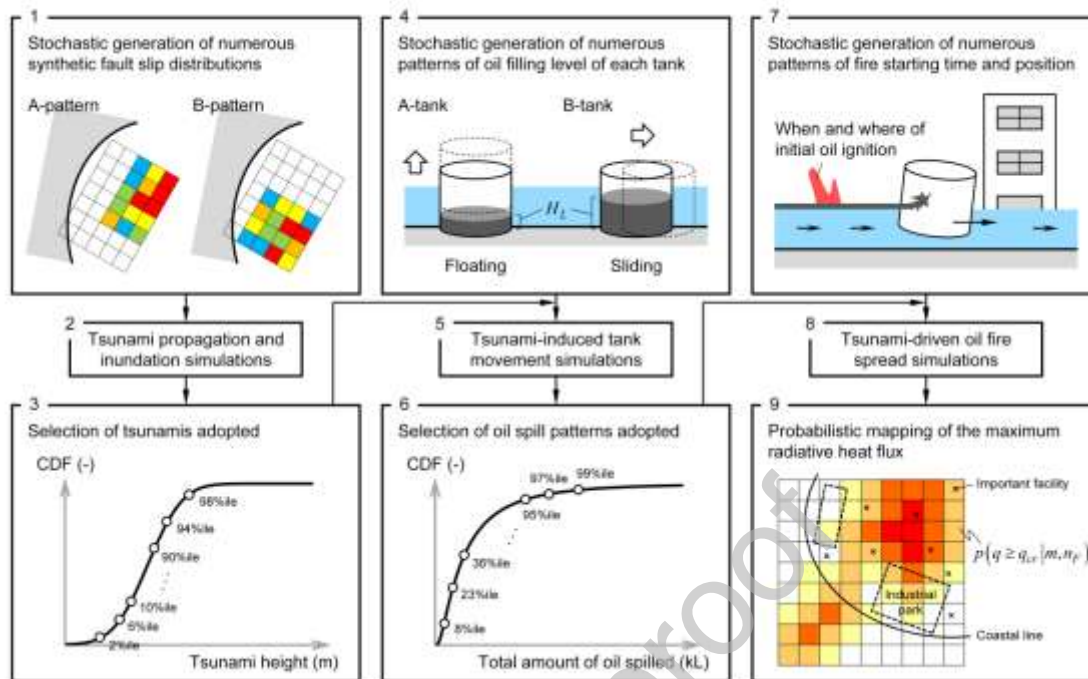
Figure 2. Computational framework for evaluating tsunami-triggered oil spill fire hazards considering associated uncertainties.
