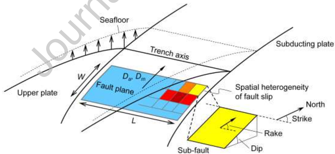
Figure 3. Schematic of a tsunami source model for a megathrust earthquake along a subduction zone.
