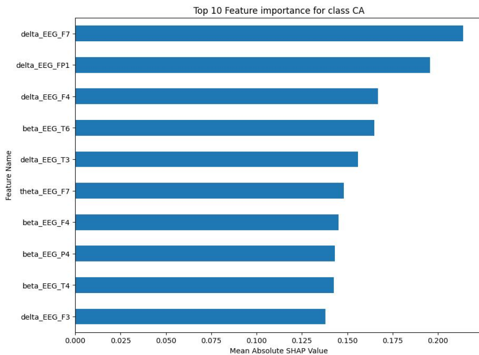
Figure 8. Top 10 important features for CA class.
