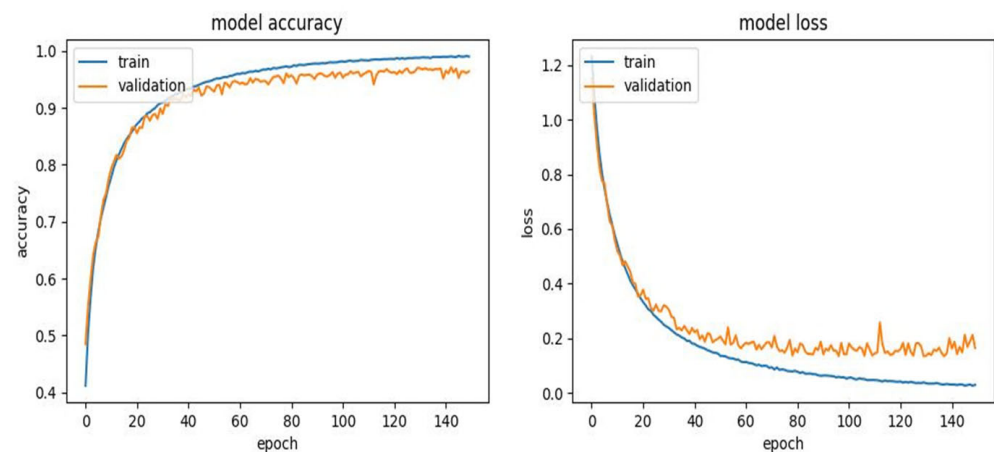
Figure 4. Training accuracy and loss curves of the proposed model.
