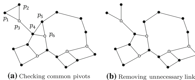
Fig. 5 Example of REMOVE- LINKS
