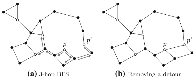
Fig. 4 Example of REMOVE- DETOURS
