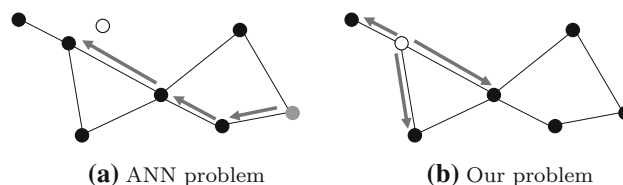
Fig. 2 Graph traversal difference between our and ANN problems (represented by arrows). Grey and white vertices respectively represent the starting object and a query object
