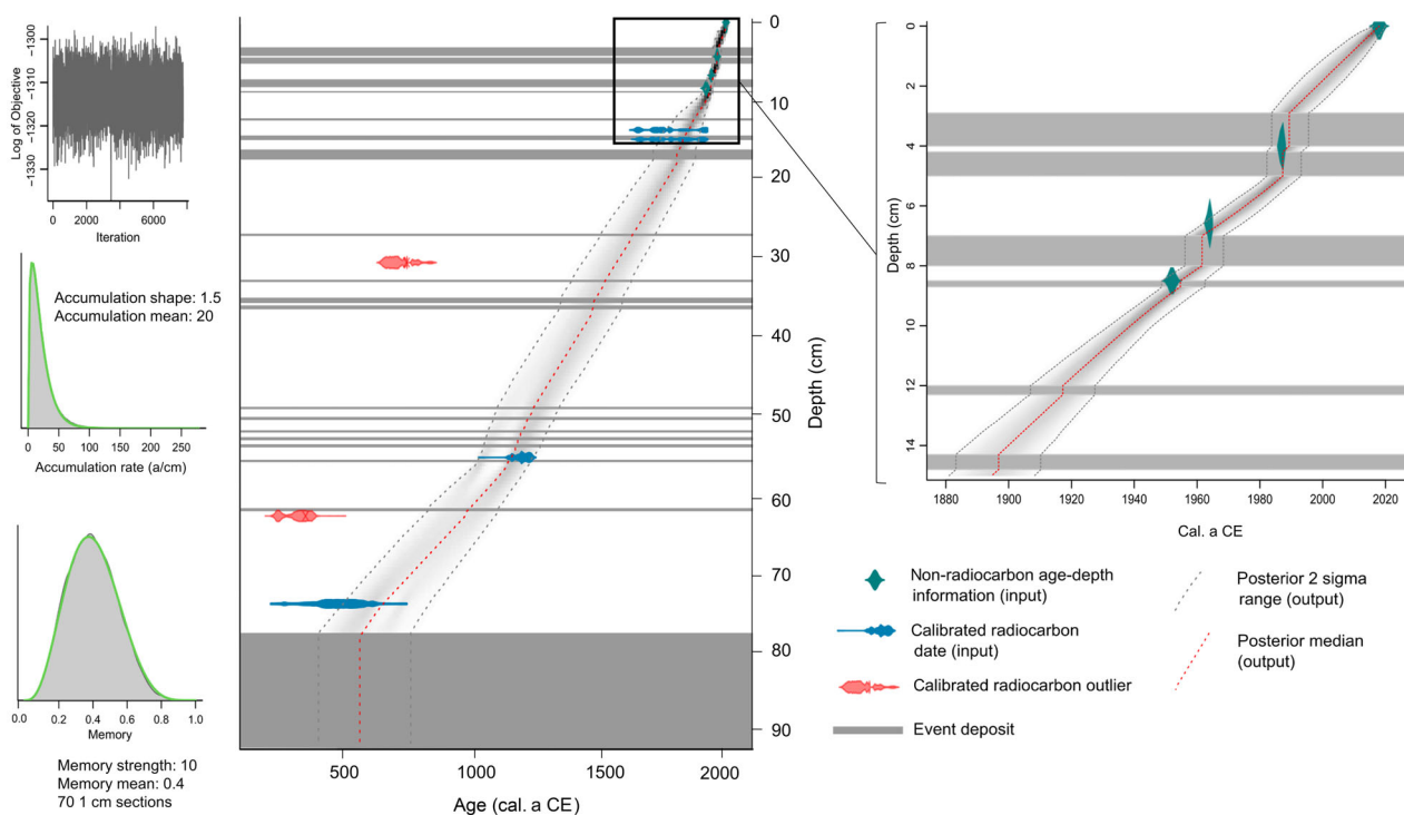
Fig. 6. rBacon-based age–depth model based on radiocarbon data (blue) and ^{13}\text{C} s data (green). The posterior age–depth model with the median (red dashed line) and the 2\sigma error range runs from bottom left to top right. The horizontal bars in the figure represent the event deposits >2 mm thick (modified after Hess et al. 2023b).
