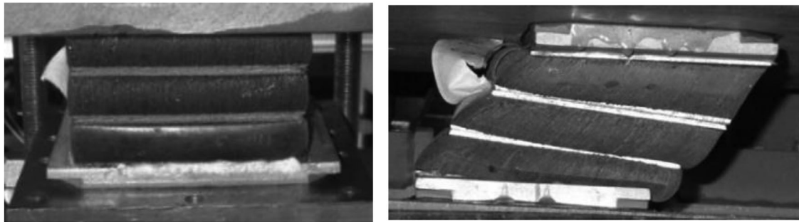
FIGURE 3 Deformed bearing under a compression load of 19 kN (left) and a combined compression load and shear displacement (right) during the experiment. 44
