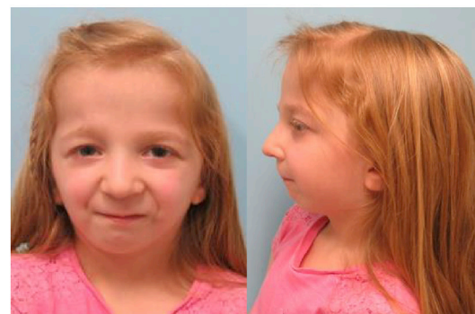
Individual 11 p.(Lys245Arg)
