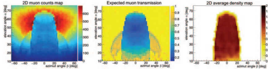
Fig. 2. – From the left: the 2D angular 2^\circ \times 2^\circ map of muon counts expected in 10 hours of data taking, the corresponding muon transmission map and the average density map without torus and external blast furnace’s skin contributions.
