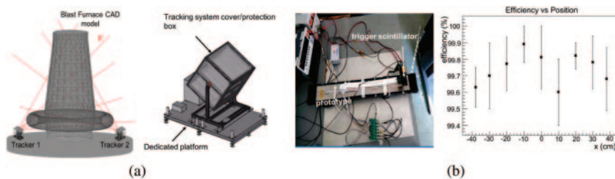
Fig. 1. – (a) Tracking system inside a protection box on the rotating platform and scheme of a possible measurement with both trackers (not in scale). (b) The experimental setup for efficiency measurements vs. muon impact point coordinate and the results (the x -axis is oriented parallel to the scintillator bars).
