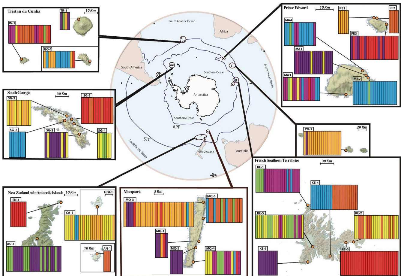
FIGURE 1 Genetic clustering of individuals within each archipelago following AMOVA-based K-means of microsatellite data. Each analysis is independent for each archipelago, and they are not related. Each bar represents one individual and colours represent genetically differentiated clusters for each archipelago. Circles around sub-Antarctic islands or nearby archipelagos represent the presence of Poa annua . Orange dots correspond to the sampled populations, each with a code given in Table 1 and Table S1 [Colour figure can be viewed at wileyonlinelibrary.com ]
