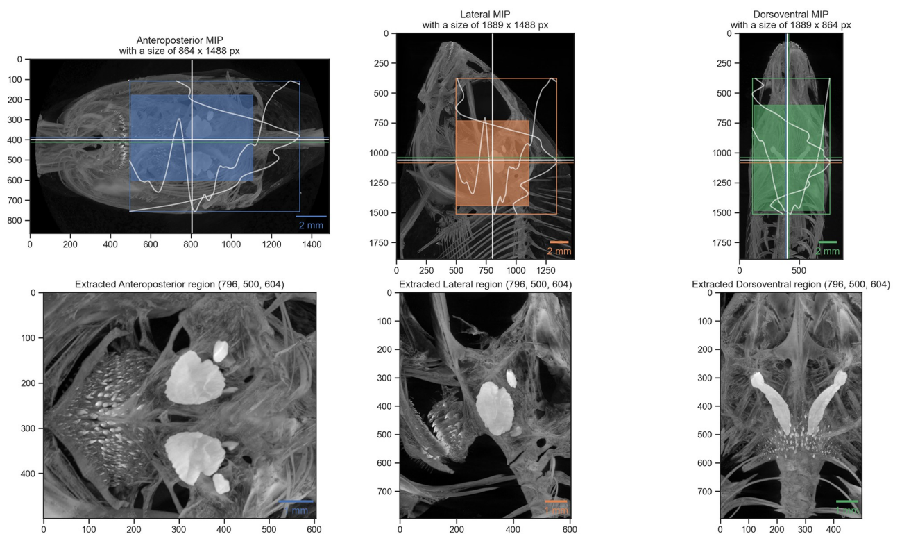
Fig 2. Visualization of automatic otolith extraction. The top row shows the found location of the otolith center in each of the three anatomical directions. The bottom row shows a maximum intensity projection of each of the three anatomical directions of the extracted otolith region.
