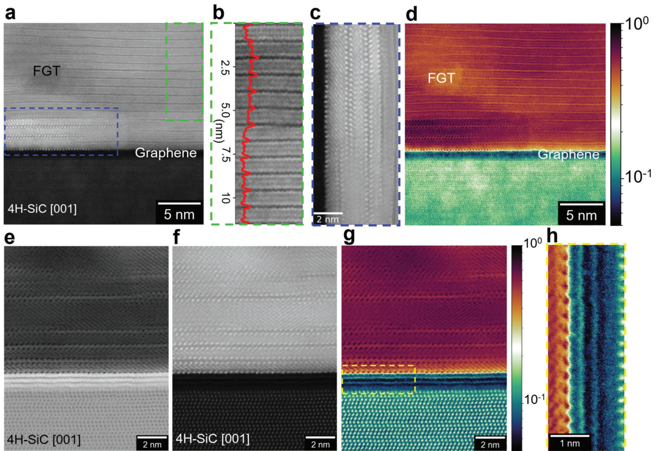
Figure 2. STEM of the 15 nm thick FGT film on graphene/SiC(0001). a) HAADF-STEM image of a region showing the FGT film on graphene. b) Magnified region from the green dashed rectangle in panel (a) showing the homogeneous layer formation and its line profile (in red). The interlayer distance is 0.97 (\pm 0.10) nm. c) Another enlarged area (blue dashed rectangle) from panel (a), showing the formation of single layers with different thicknesses. d) The same image as in panel (a) rendered using a custom colormap to aid visualization. e) Bright field-STEM image showing another region of the sample where the graphene layers are better resolved. f) HAADF-STEM image of the same area in panel (e). g) Colormap version of the same area in panel (e) to aid visualization of the graphene layers. h) Enlarged region of the yellow rectangular box in panel (g).
