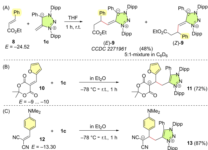
Scheme 4. Reactivity of mNHOs 1 towards Michael acceptors (A) 8 , (B) 10 and (C) 12 (yields refer to isolated products).
