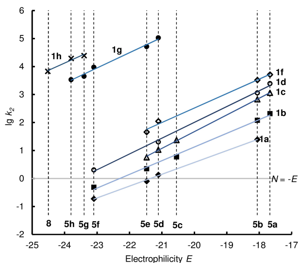
Figure 3. Linear relationships of \lg k_2 of reactions of mNHOs 1a–h with the reference electrophiles 5 (and 8 ) in THF at 20 °C with the electrophilicity parameters E of 5 (and 8 ); the correlation for 1e is shown in the Supporting Information.
