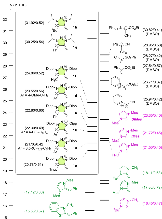
Figure 5. Embedding mNHOs 1a–h in the nucleophilicity scale ( N/S_N values in parentheses were taken from ref. [18] and refer to reactions in THF if not indicated otherwise).
