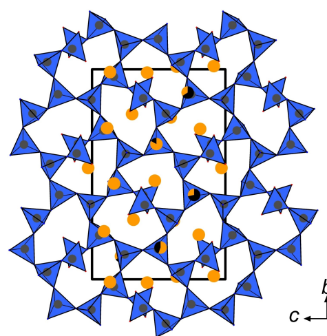
Figure 2. Crystal structure of \text{La}_7\text{Sr}[\text{Si}_{10}\text{N}_{19}\text{O}_3] . \text{Si}(\text{N},\text{O})_4 tetrahedra in blue, Si atoms dark gray, La atoms orange, Sr atoms black. Mixed occupied cation sites colored in the respective atom colors with the section size corresponding to the percentage occupancy.
