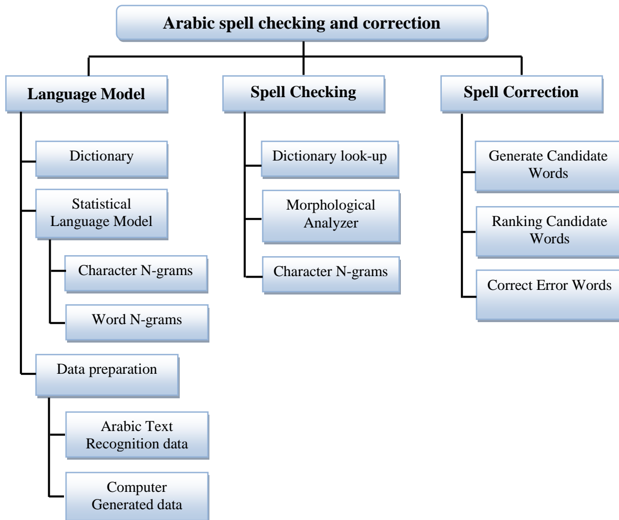
Figure 4.2 Implementation structure of Arabic Spell Checking and Correction
