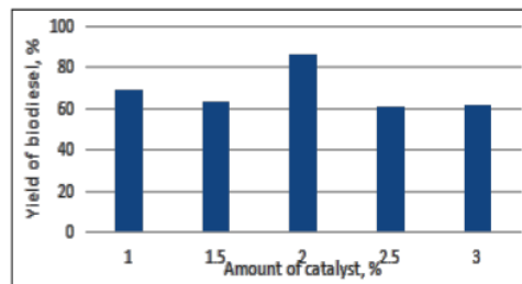
Fig. 3. Biodiesel yield on various catalyst concentrations
