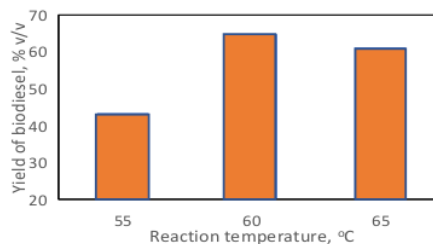
Fig. 2. Yield of biodiesel at difference temperature [29]
