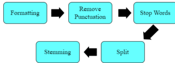
Fig. 4. Preprocessing
