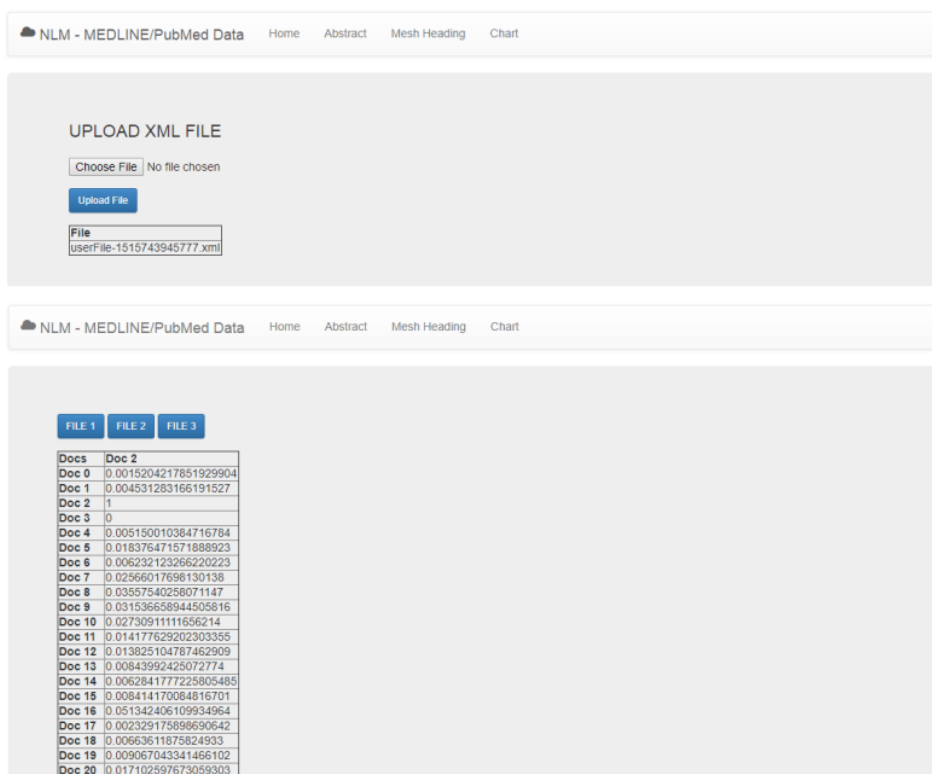
Fig. 5. PubMed application
