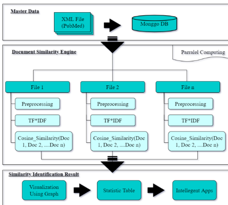
Fig. 1. The Similarity identification framework
