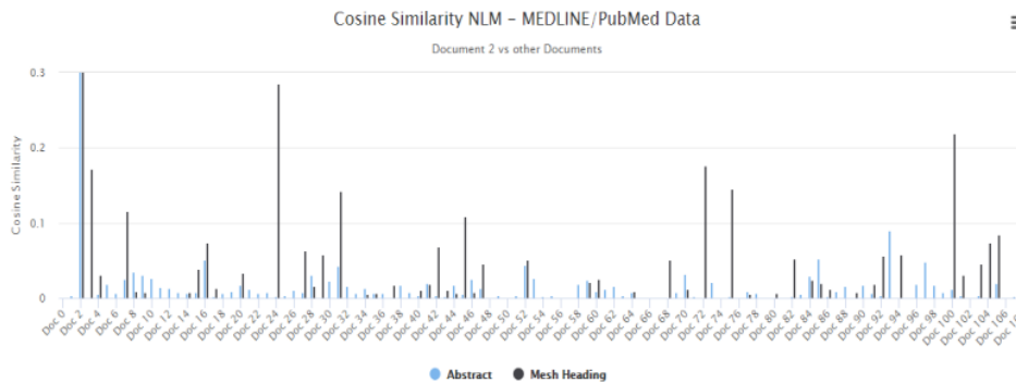
Fig. 10. Visualization of comparison of cosine similarity result between documents
