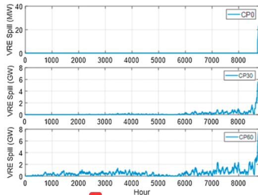
Fig. 4. Energy spills from least-cost mix solutions with VRE for each CP at 0.005 % upper USE limit and without any reserve requirement.
