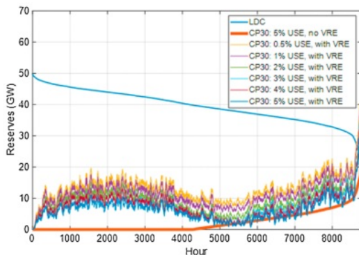
Fig. 8. System operating reserves curves of least-cost mix with VRE vs LDC at 0.5% - 5% upper USE limit and without reserves requirement for CP30, and their comparison with reserves curve without VRE at 5% upper USE limit.
