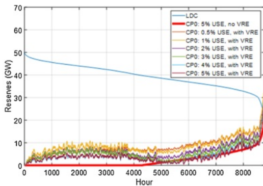
Fig. 7. Operating reserves curves of least-cost mix with VRE vs LDC at 0.5% - 5% upper USE limit and without reserves requirement for CP0 and their comparison with reserves curve without VRE at 5% upper USE limit.
