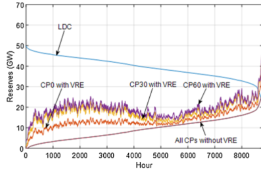
Fig. 3. Operating reserves curves of least-cost mix with and without VRE vs LDC with 0.005 % upper USE limit and no reserves requirement for all CPs.
