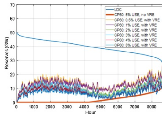
Fig. 9. System operating reserves curves of least-cost mix with VRE vs LDC at 0.5% - 5% upper USE limit and without reserves requirement for CP60, and their comparison with reserves curve without VRE at 5% upper USE limit.
