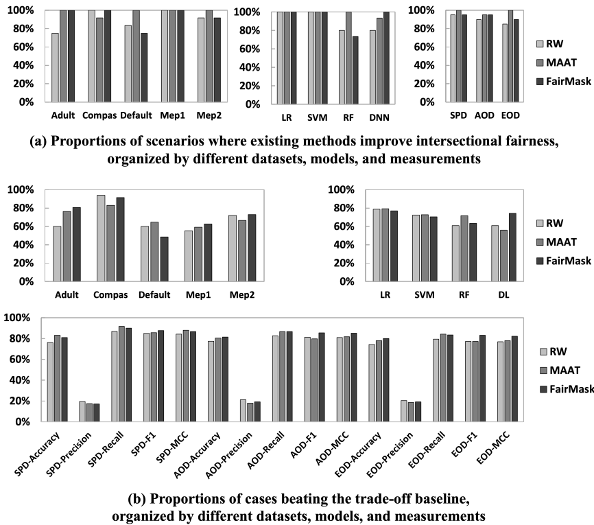
Figure 2: (RQ4) Effectiveness in intersectional fairness improvement and fairness-performance trade-off of the best three methods identified in this study (i.e., RW, MAAT, and FairMask) across various datasets, models, and measurements. We observe that it is challenging for these methods to achieve a good fairness-performance trade-off for imbalanced datasets and precision-critical applications.
