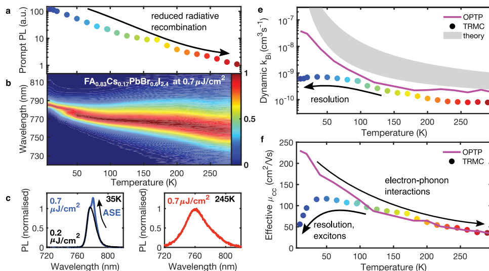
Figure 2. Temperature-dependent optoelectronic properties of a thin film of \text{FA}_{0.83}\text{Cs}_{0.17}\text{PbBr}_{0.6}\text{I}_{2.4} perovskite. a) Prompt PL intensity—the intensity at the time immediately following photoexcitation, for PL transients shown in Figure S2, Supporting Information, shown as a function of temperature. The color of the data points corresponds to the color of the traces shown in the Supporting Information. b) The corresponding time-integrated emission spectra normalized at their peak as a function of temperature. Example spectra for the sample lattice temperature of c) 35 K and d) 245 K, with the spectrum of the perovskite at low temperature also showing the appearance of a narrowed amplified spontaneous emission peak at high excitation fluence. e) Bimolecular recombination rate constant k_{\text{Bi}} as a function of temperature, extracted from fits to microwave photoconductivity decays (colored dots, from decays shown in Figure S1, Supporting Information) and to THz photoconductivity transients (magenta line, from decays shown in Figure S7, Supporting Information). The grey shaded area shows the behavior predicted from detailed-balance models, in the presence or absence of Coulombic interactions (top and bottom bound, respectively) according to Ref. [48]. f) The extracted effective electron–hole sum mobility, \phi\mu_{\text{cc}} , obtained from microwave (dots) and THz (magenta line) photoconductivity decay traces.
