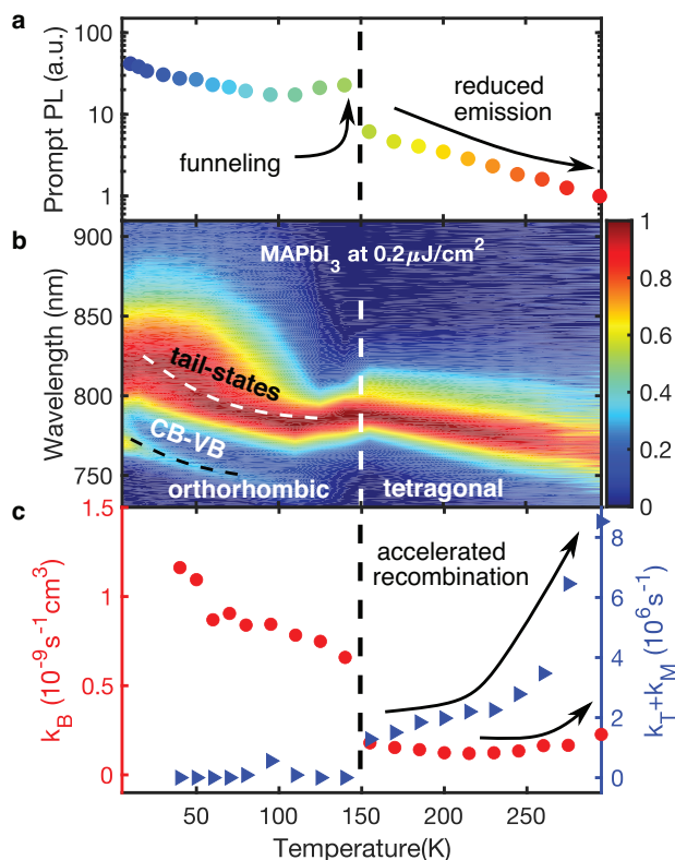
Figure 3. Temperature evolution of emission and conductivity of a MAPbI 3 thin film: a) prompt PL intensity, b) emission spectrum, and c) dynamic decay rates, with the phase transition indicated by a dotted line around 150 K. The prompt PL intensity was extracted from PL transients shown in Figure S4, Supporting Information. The bimolecular and monomolecular decay constants were extracted from fits of the model described by Equations (1a) and (1b) to microwave conductivity transients shown in Figure S3, Supporting Information. The value of k_M + k_T represents the total monomolecular recombination rate of charge carriers.
