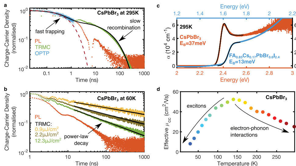
Figure 4. Optoelectronic properties of a thermally evaporated CsPbBr 3 perovskite thin film. a) Room-temperature charge-carrier decay dynamics, represented by the decay of THz photoconductivity (open blue circles), MW conductivity transients (green dots), and photoluminescence signal decay (square root of intensity, shown as orange dots). The black solid line represents the fit to the conductivity data resulting from the model described in the main text. The dashed red line shows the predicted transient of the PL intensity. b) Microwave photoconductivity decays at 60 K, shown in yellow, brown, and green dots for different excitation fluences indicated by legend colors matching those of the datapoints. The square root of PL intensity is shown in orange dots. Black solid lines show power-law fits to the microwave data. c) Absorption onsets of CsPbBr 3 and FA 0.83 Cs 0.17 PbBr 0.6 I 2.4 at room temperature, shown as orange and blue dots, respectively. Black lines show fits according to the Elliott function [89] and the extracted exciton binding energies are indicated in the color matching that of the datapoints. d) Dependence of effective electron–hole sum mobility on temperature, extracted from microwave photoconductivity traces (as outlined in Section S4.1, Supporting Information) shown as solid dots, whose colors match those of the conductivity transients presented in Figure S5, Supporting Information.
