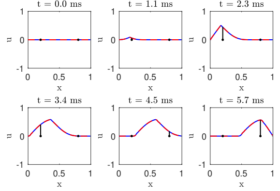
Figure 5: Time evolution of a string under the influence of N_s = 2 nonlinear springs (represented as black lines). Solid blue: scheme (35); dashed red: Störmer-Verlet. Here, the string has a fundamental frequency of 100 Hz, a mass of 1 g, and presents a total M = 128 modes between the fundamental and the limit of stability. The string is activated using a strike with T_e = 5 ms, f_{e,max} = 200 N. The springs are located at 0.2L , 0.8L , and have K = 7.3 \cdot 10^{-4} , \gamma = 1.1 , \beta = 0 . For this simulation, \epsilon_0 = 10^9 .
