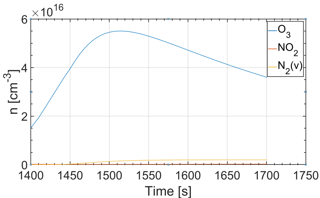
Figure 15. Temporal evolution of the number densities of ozone, \text{NO}_2 and vibrationally excited nitrogen molecules during the second ignition of the SDBD reactor, considering an input power of 35 W.
