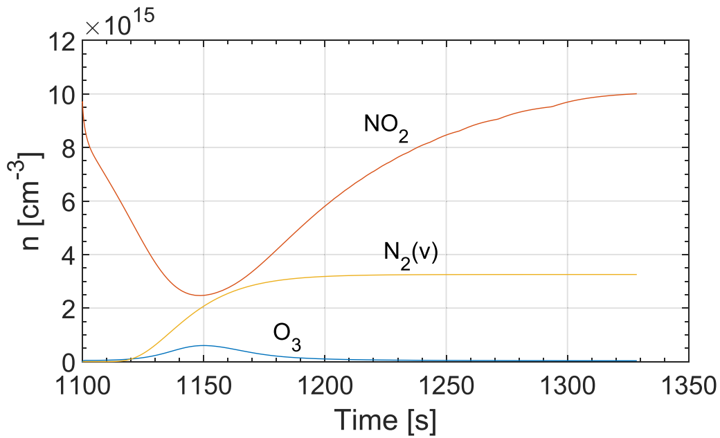
Figure 14. Temporal evolution of the number densities of ozone, \text{NO}_2 and vibrationally excited nitrogen molecules during the second ignition of the SDBD reactor, considering an input power of 100 W.
