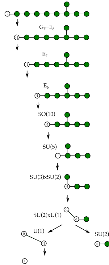
Fig. 1. CFD-transition tree for rank one 5d SCFTs including the superconformal flavor symmetries G_F .
