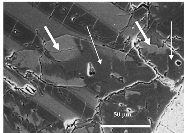
Fig. 4. (a) BSE image of the AC-BO-214/3 chondrule (PTS Acfer 214 Algerien). Rectangular areas A1–A2 are the selected areas for point counting, as explained in the text. (b) Detail BSE image of the area indicated in part (a), showing the pyroxene with crystal faces against the glass. Arrows (thick and thin) indicates high and low-Ca pyroxene, respectively. (c) SEM Al image of part (b), which clearly shows how the surface of the olivine lath close to the pyroxene is retracting toward the center of the original plate. Arrow indicates glass inclusions in the form of a straight line in the center of the olivine plate. (d) SEM Mg image of part (b), where the wedge of the olivine, where overgrown by the pyroxene, is clearly observed. (e) SEM Ca image of part (b), showing the Ca-rich border of the pyroxene.
