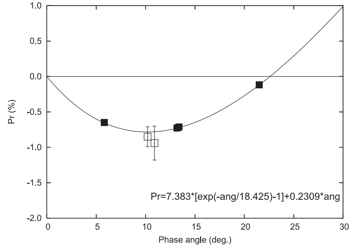
Fig. 4. Polarimetric observations of 347 Pariana. Filled marks are data taken during this campaign.
