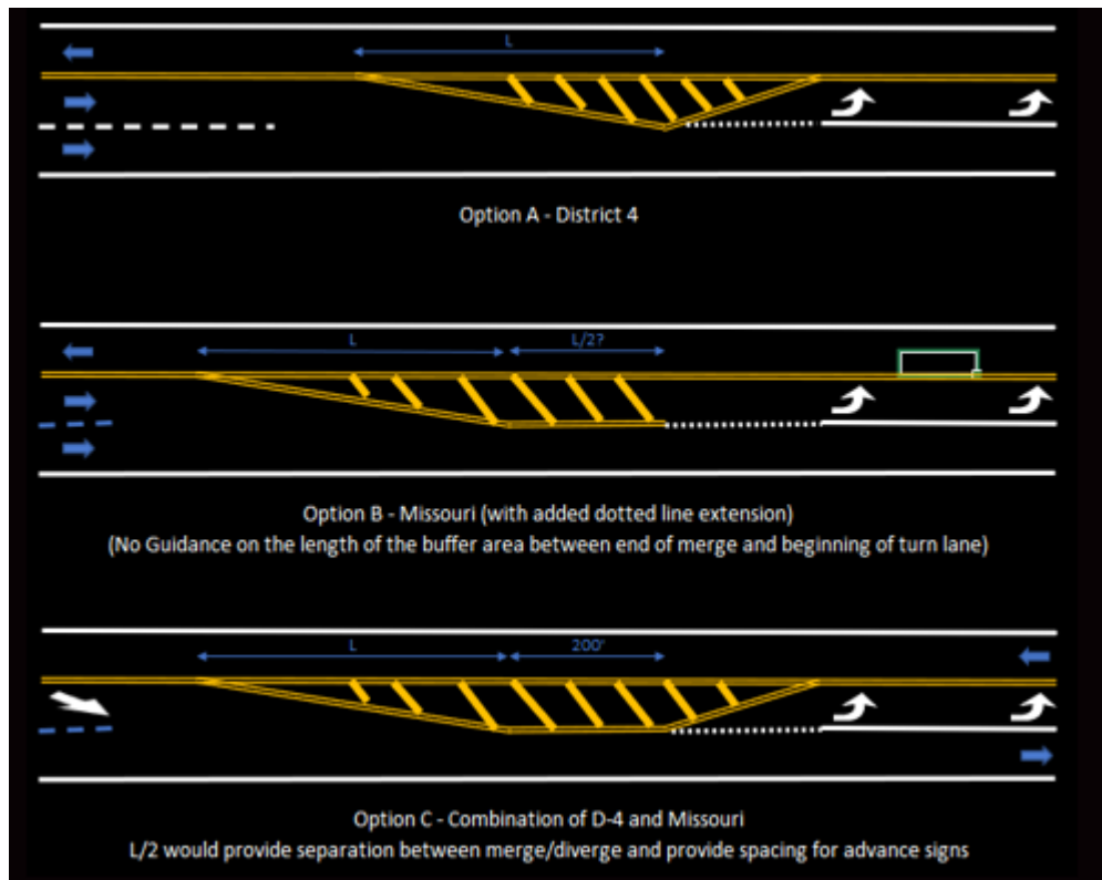
Figure 2.11 Markings for Transitions to Intersection, Passing Lane Approaching Left-Turn Lane
