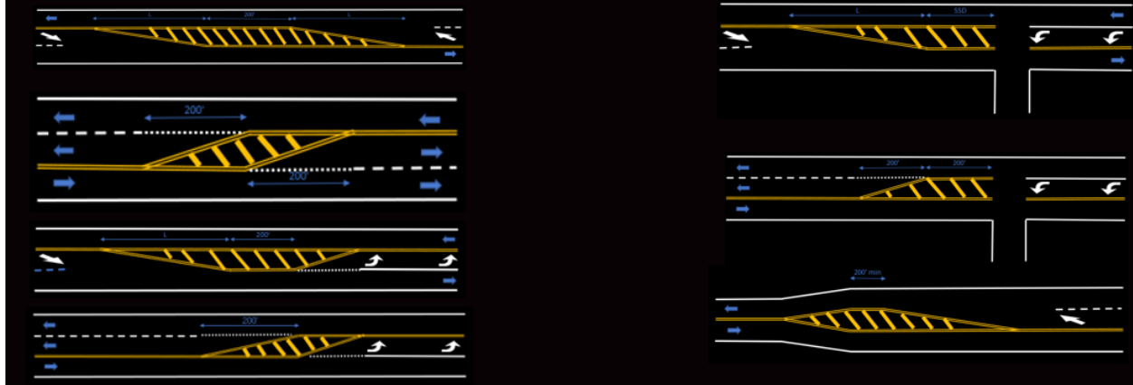
Figure 5.4 Preferred Marking Locations for Common Scenarios
