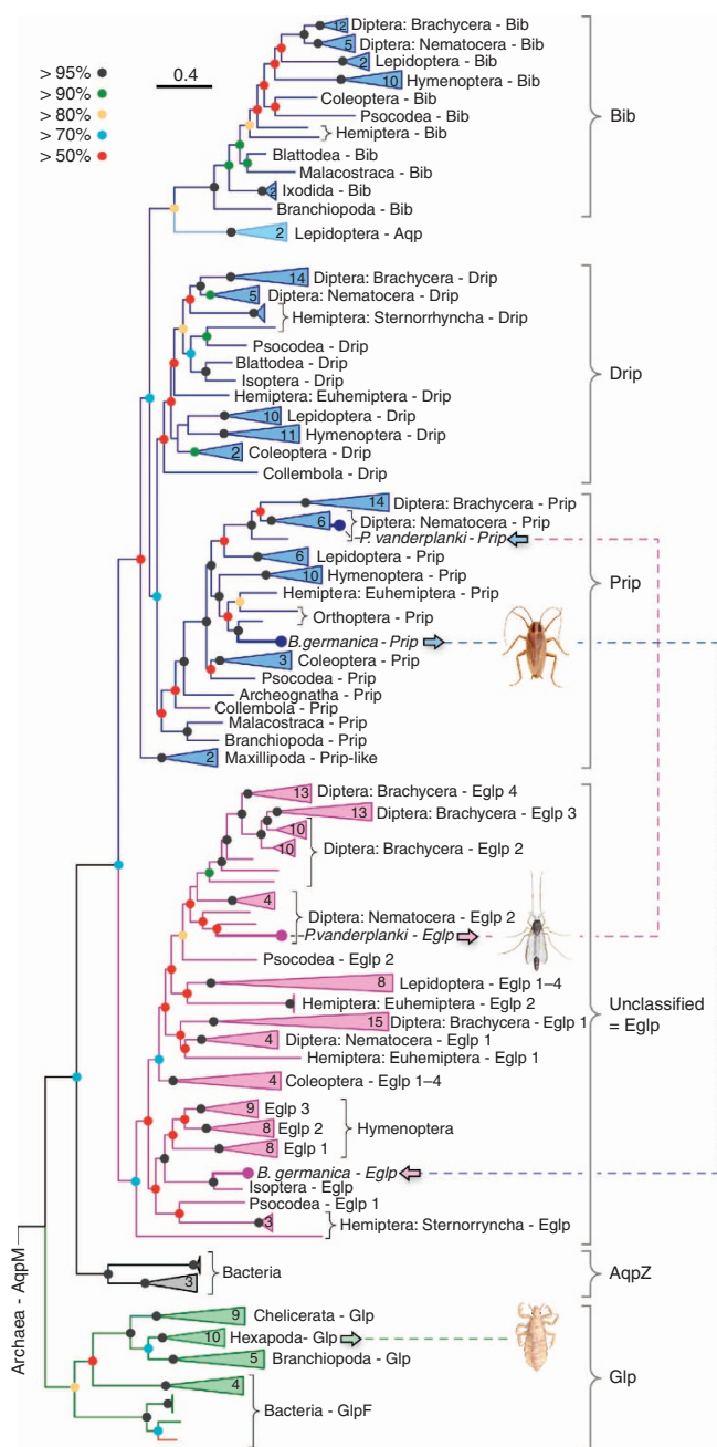
Figure 1 | Molecular phylogeny of arthropod orthodox aquaporins.
