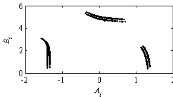
Figure 3. RM for traditional CSK scheme when \beta switched in two values.
