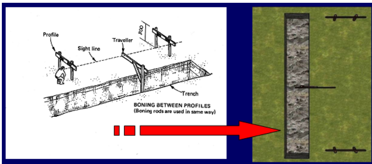
FIG. 5: Visualisation of traveller and sight rails.
