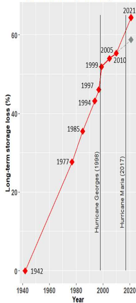
Lago Dos Bocas Long-Term Storage Loss
