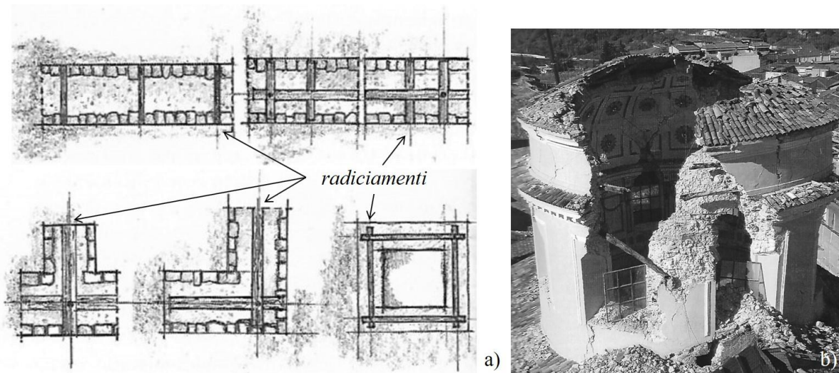
Figure 4: The wooden anti-seismic technique diffused in L’Aquila, known as “radiciamenti”: a) wooden frames with different structural functions and b) the 3 orders of “radiciamenti” visible in the partially collapsed dome of Santa Maria del Suffragio hit by the 2009 L’Aquila earthquake (source from [11], pp. 27 and 52).
