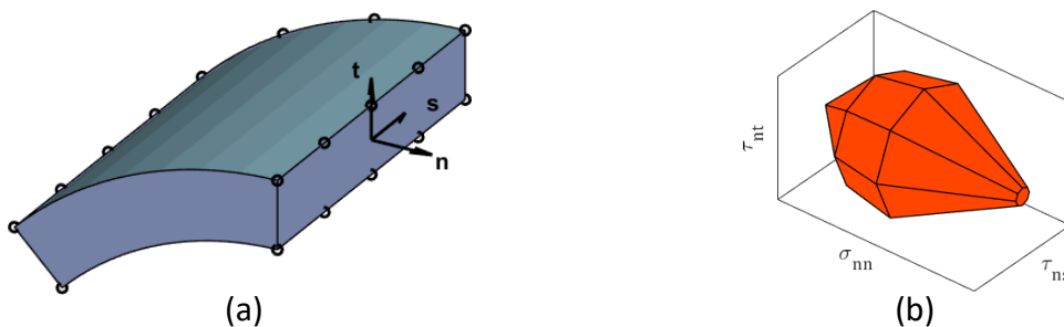
Figure 3. Representation of masonry behavior: masonry-masonry interface and corresponding local reference system (a), and linearized 3D representation of the failure domain (b).
