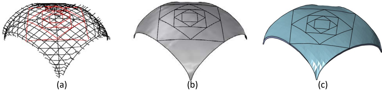
Figure 5. Construction of the NURBS model of the single vault: (a) section lines, (b) assembly of NURBS surfaces in Rhinoceros and (c) obtained NURBS model in MATLAB.
