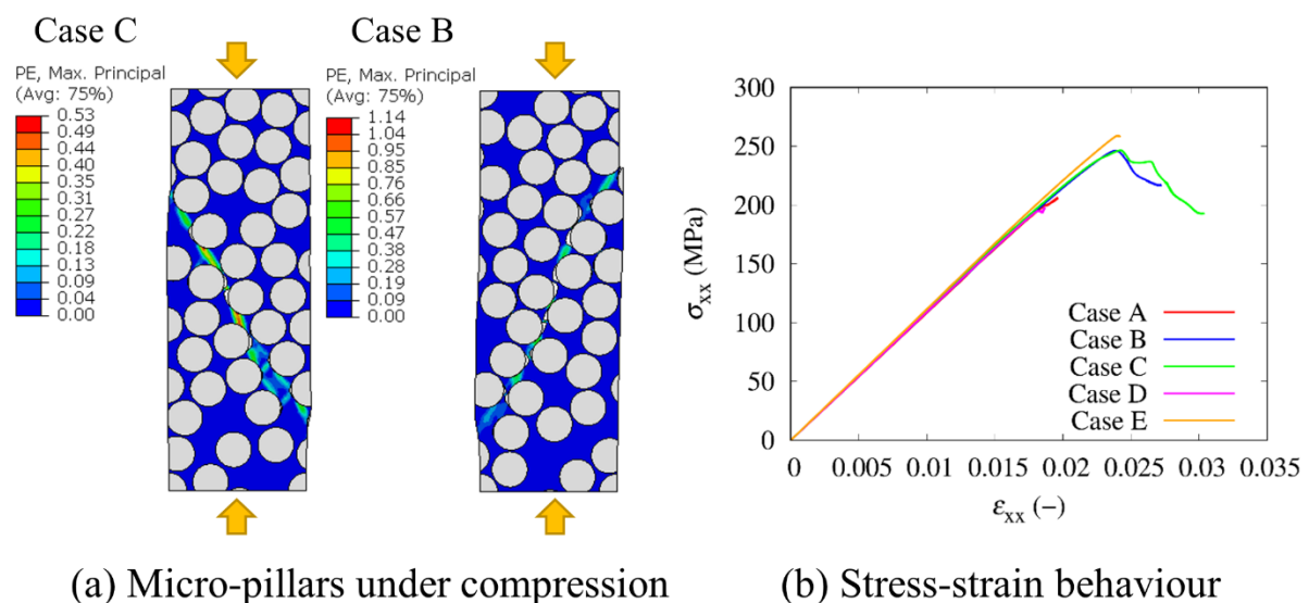
Figure 1. (a) Maximum principal plastic strain field of two micro-pillar under compression, and (b) the stress-strain behaviour of different micro-pillars with same dimensions and volume fraction.
