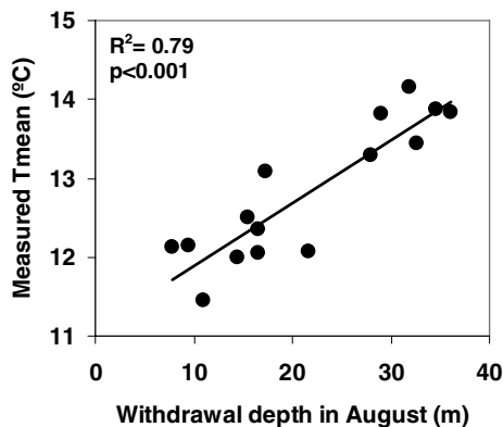
Figure 7. Relationship between measured T_{\text{mean}} and withdrawal depth in August ( Z_{\text{out August}} ). Solid line represents Equation (6) in the text.
