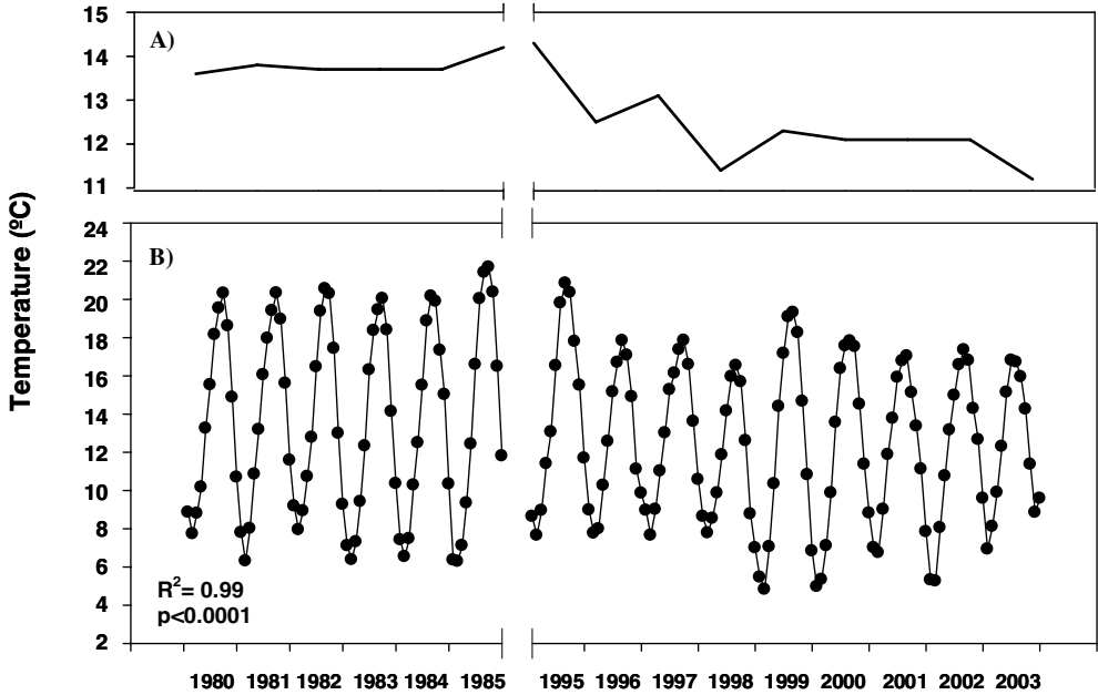
Figure 5. A) Mean annual water temperature recorded in Sau Reservoir along the 1980–2003 period. B) Monthly average temperature in Sau Reservoir water column during the study period. Black dots represent the simulated temperature values with Equations (6) and (7). R^2 and P -values correspond to the observed-simulated data correlation.
