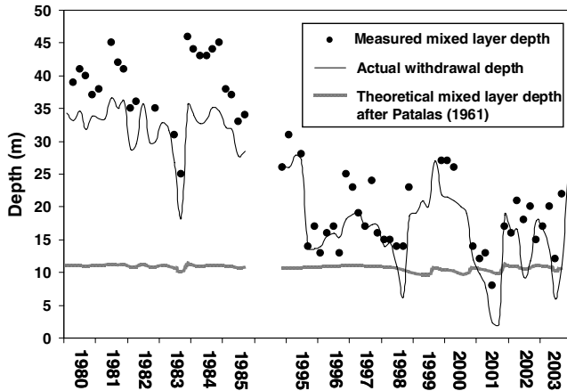
Figure 10. Temporal trend of the mixed layer depth ( Z_{\text{mix}} , black dots) and the selective withdrawal depth ( Z_{\text{out}} , solid line) in Sau Reservoir during the study period. The grey bold line depicts the hypothetical mixed layer depth if Sau behaved as a lake, computed from morphometric features following PATALAS (1961).
