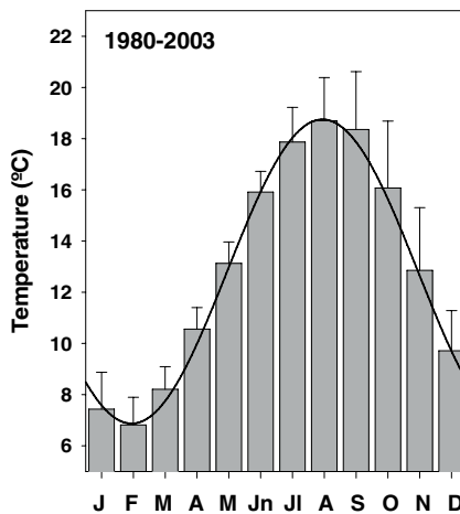
Figure 6. Mean monthly water column temperature for an average year of the 1980–2003 period. Continuous line represents the sinusoid function fitted for empirical modeling (Equation (7)).
