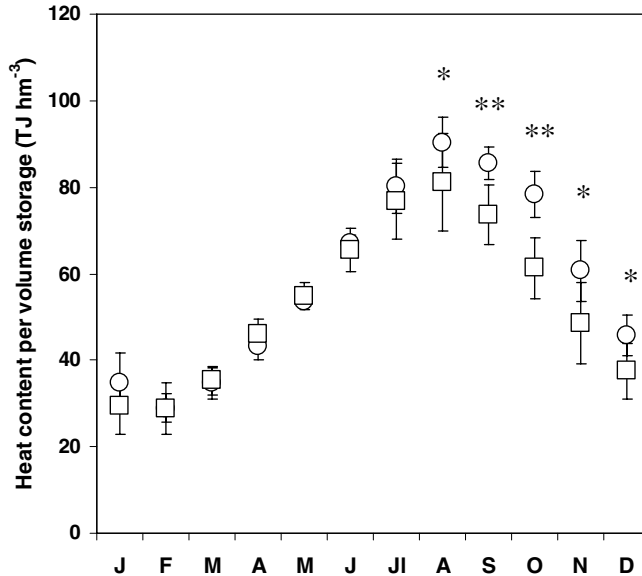
Figure 4. Results of a non-parametric Kruskal-Wallis test on the mean monthly heat content per volume storage from the two studied periods. Circles: 1980–1985; Squares: 1996–2003. * significant differences at P < 0.05 ; ** significant differences at P < 0.01 .
