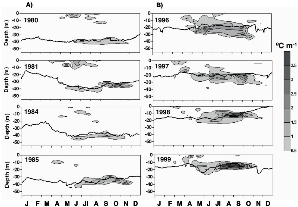
Figure 1. The annual development of the seasonal thermocline (expressed as temperature gradients) (A) for a selected set of years during the 1980–1985 period, when hypolimnetic withdrawal resulted in a deep thermocline and a wide metalimnion, and (B) for a selected set of years during the 1996–2003 period, when epilimnetic water flowed through the intermediate outlet inducing the development of a shallower thermocline. The solid black line depicts the daily development of the withdrawal depth.
