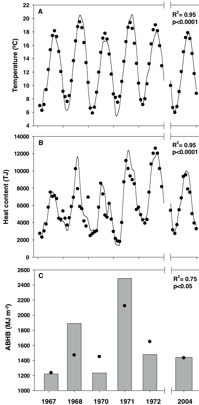
Figure 9. Model validation for A) water temperature, B) heat content, and C) ABHB. Points are measured values, lines and bars are modeled values.
