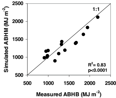
Figure 8. Relationship between measured and simulated ABHB in Sau Reservoir. Solid line represents the 1:1 regression.
