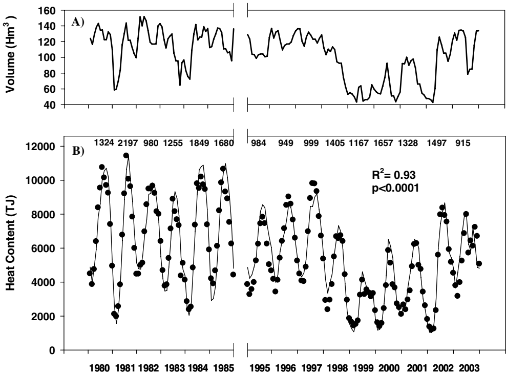
Figure 3. A) Monthly water volume recorded in Sau Reservoir during 1980–85 and 1995–2003 periods. B) Monthly heat content in Sau Reservoir during the studied period. Bold numbers in the top depict the ABHB ( \text{MJ m}^{-2} ). Black dots represent the simulated heat content values with Equations (6) to (9). R^2 and P -values correspond to the observed-simulated data correlation.
