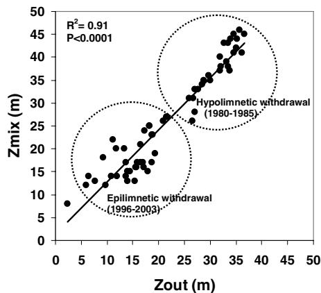
Figure 2. The relationship between the water extraction depth ( Z_{out} ) and the mixed layer depth ( Z_{mix} ) in Sau Reservoir. Solid line represents Equation (5) in the text.
