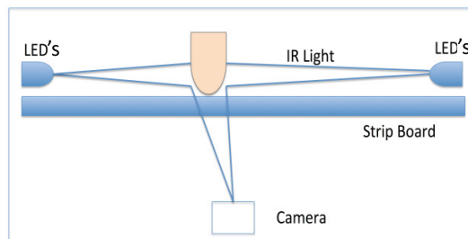
Fig. 4. Light from the infrared LED's is reflected through the strip board when it is touched
