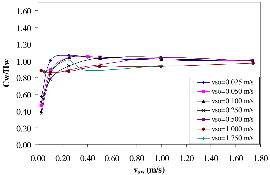
Figure 50 - Experimental Water Holdup Ratio ( +2^\circ Upward)
