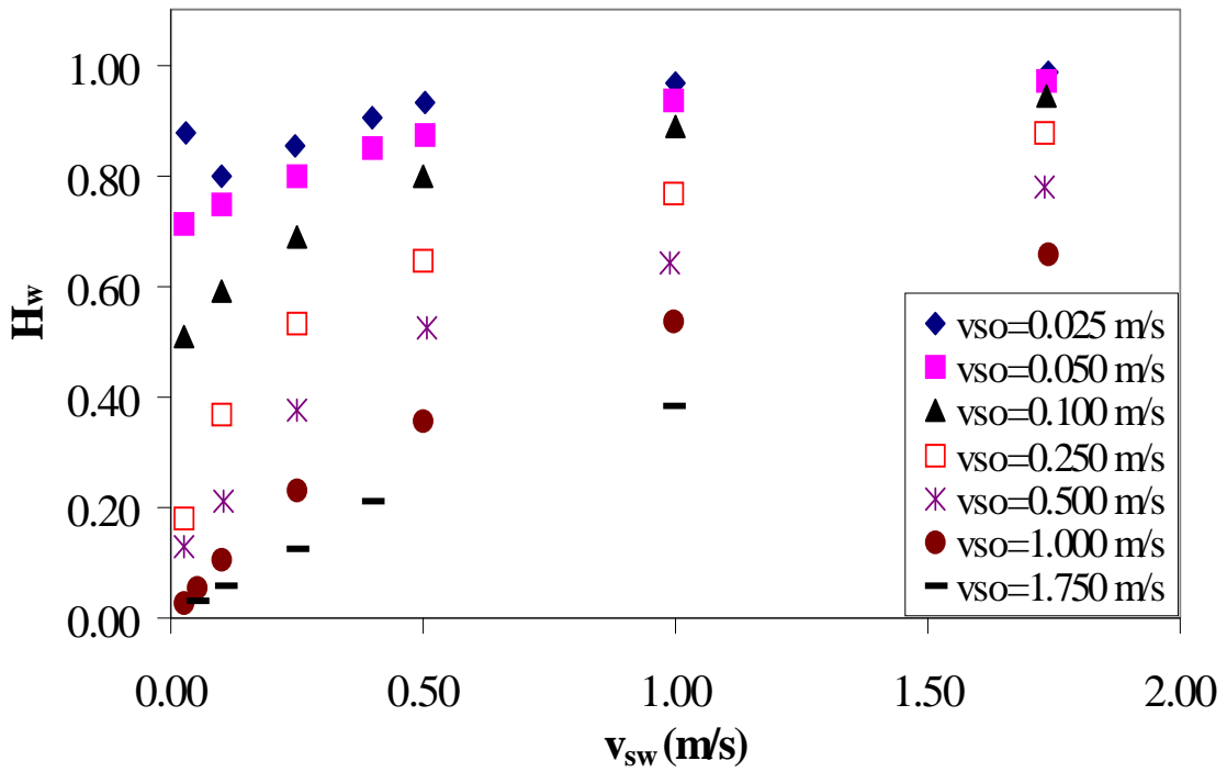
Figure 49 - Experimental Water Holdup ( +2^\circ Upward)
