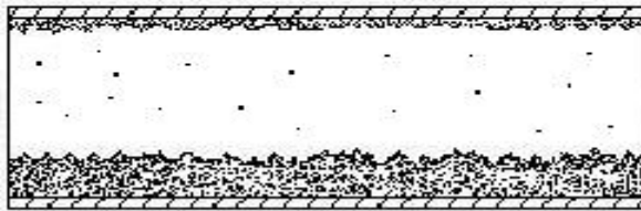
Figure 19 - Annular-Oil Continuous (AN-OC) and Annular -Water Continuous (AN-WC) Gas-Oil-Water Flow Patterns
