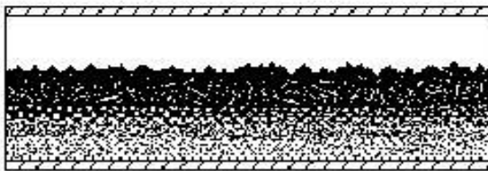
Figure 15 - Stratified-Stratified (ST-ST) and Stratified-Dual Continuous (ST-DC) Gas-Oil-Water Flow Patterns
