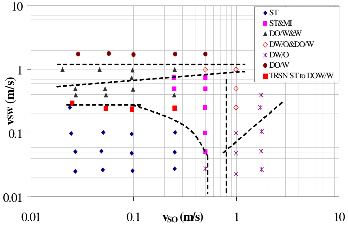
Figure 28 - Experimental Flow Pattern Map (-1° Downward)
