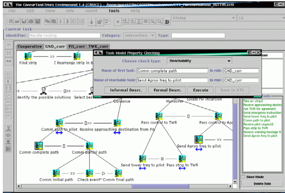
Fig. 6. Interactive Composition of a Property.
