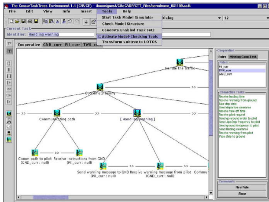
Fig. 3. Activation of the model checking tools.
