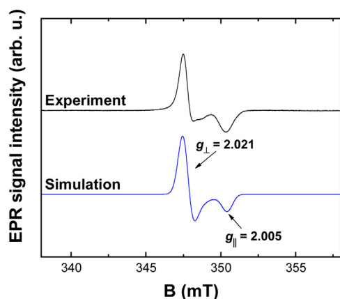
Fig. 17. Simulation of the Nafion® EPR spectrum after a 500 kGy irradiation dose.
