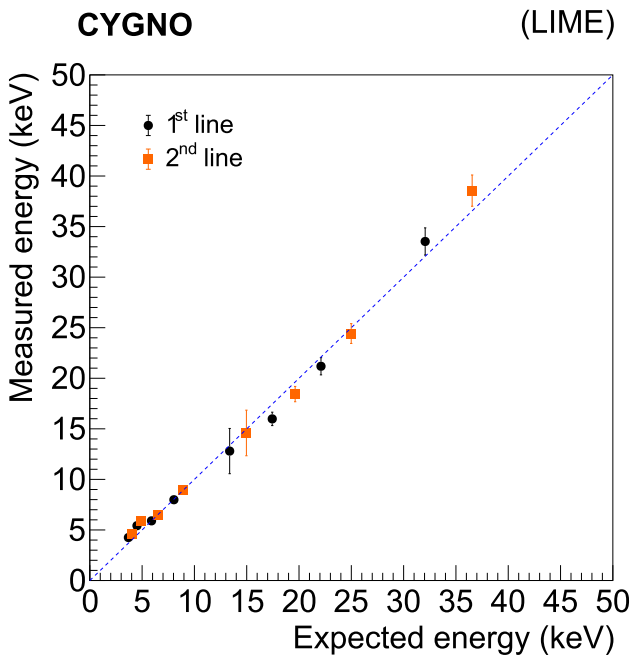
Fig. 18 Estimated average energy response versus the expected one from the K_\alpha (black dots) or K_\beta lines contributions. The uncertainties on each point represent the statistical contribution and the systematic uncertainty arising from the knowledge of the z position. The dotted line represents a perfect linear response of the detector
