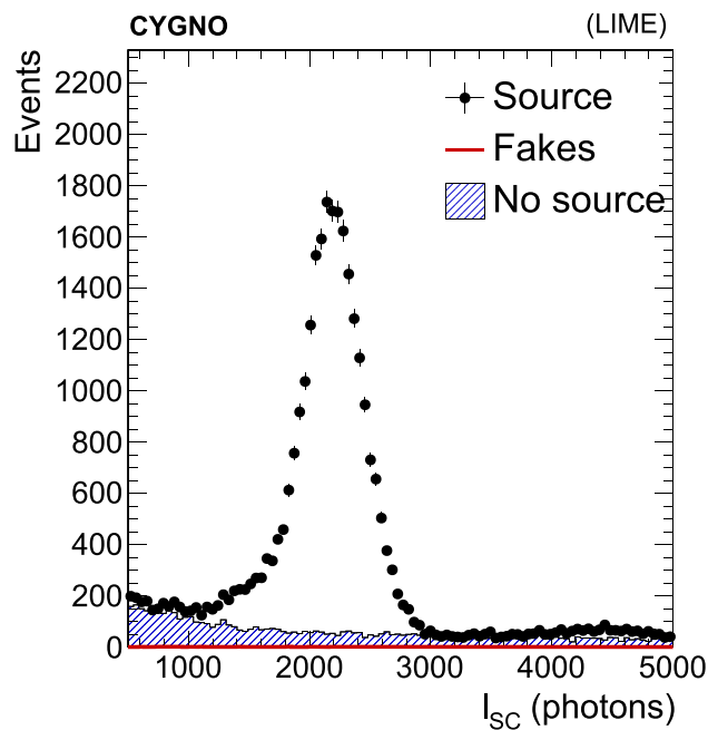
Fig. 10 Light integral I_{SC} of the reconstructed clusters, as defined in the text. Top (bottom): region below (around) the expected energy peak from X-rays interactions from the ^{55}\text{Fe} source. Black points represent data in presence of the ^{55}\text{Fe} source, filled histogram represents data without the source, while the red hollow histogram represents the contribution from mis-reconstructed clusters from the electronics noise. The latter two are normalized to the live-time of the data taking with the ^{55}\text{Fe} source
