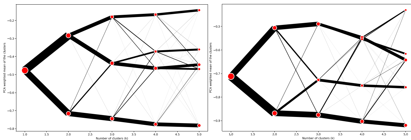
FIGURE 3 Illustrative clustergrams for 1 to 5 cluster solutions for Supergroup 1 and for Group 1b.
