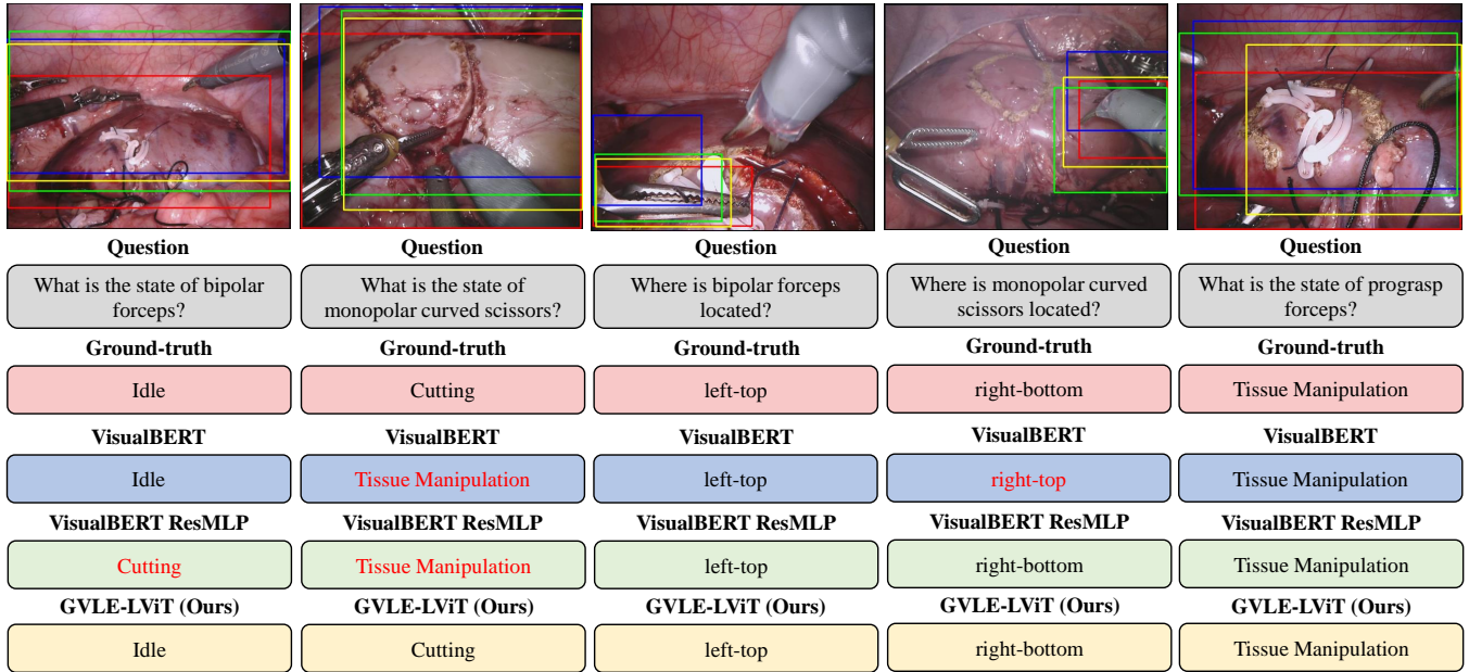
Fig. 3. Several examples of answer and bounding box generation by VisualBERT [9], VisualBERT ResMLP [2], and our GVLE-LViT model. Compared with the baseline models, the localization and classification prediction results of our model are more accurate. The denotation of bounding box color is as follows: red: Ground-truth, blue: VisualBERT [9], green: VisualBERT ResMLP [2], yellow: GVLE-LViT (Ours).
