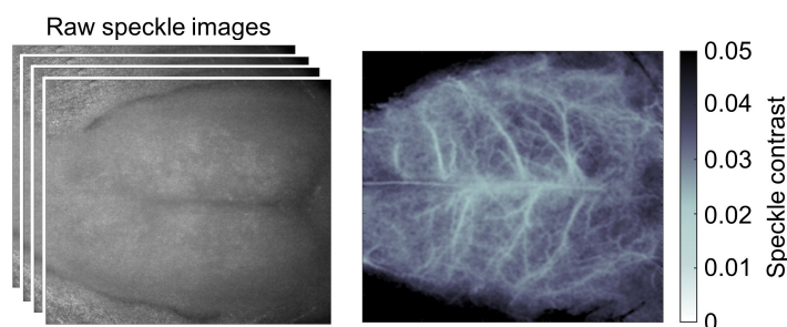
Figure 1. Raw speckle and processed images of the rat brain obtained transcranially.
