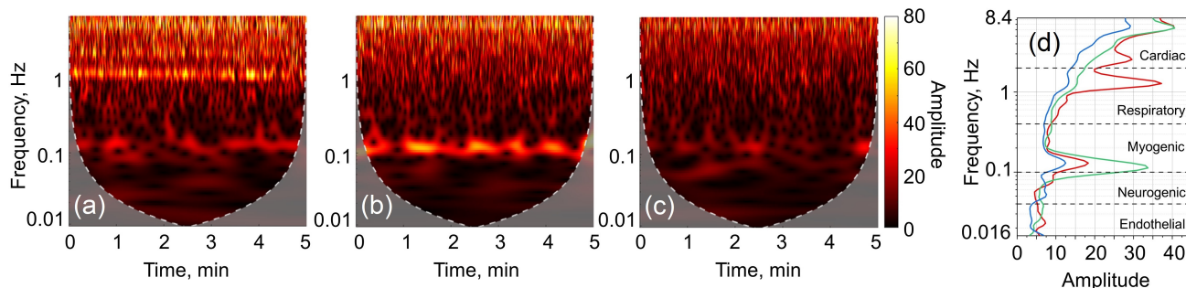
Figure 2. Wavelet analysis of obtained perfusion values: (a) CWT amplitude scalogram for the superior sagittal sinus (red line in d), (b) tributary (green line in d), and (c) brain tissue that does not have clearly visualized vessels (blue line in d); (d) time-averaged spectra for data obtained in the aforementioned ROIs.
