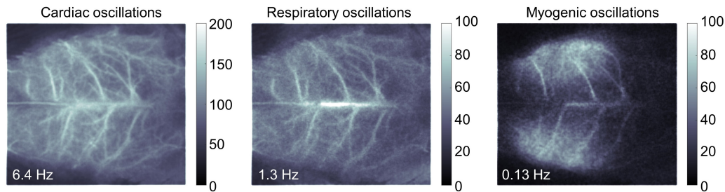
Figure 3. Spatial variations in cardiac (6.4 Hz), respiratory (1.3 Hz), and myogenic (0.13 Hz) activity.
