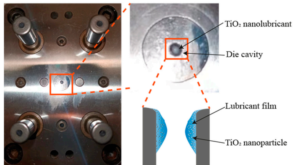
Figure 2. Application of TiO 2 nanolubricant in MDD experiments.
