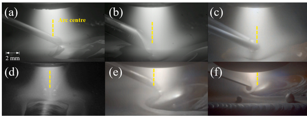
Fig. 8. Process images of wire melting behaviours for the five wire configurations: (a) 1.2 mm Ti wire; (b) 2.4 mm Ti wire; (c) dual Ti wire (longitudinal view); (d) dual Ti wire (lateral view); (e) 1.2 mm MS wire; (f) flat MS wire.
