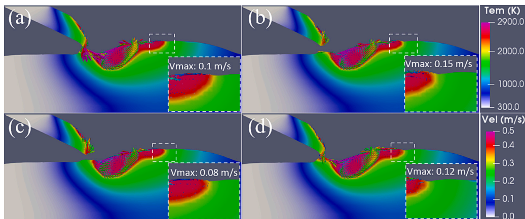
Fig. 14. Longitudinal central slices of fluid flow in the melt pool during a quasi-steady state (after 3.0 s) for the 2.4 mm Ti wire: (a) 3.1906 s; (b) 3.2146 s; (c) 3.2386 s; (d) 3.2866 s.
