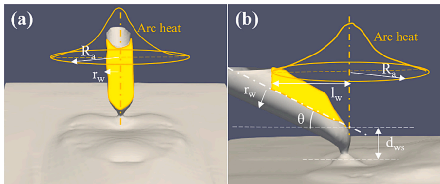
Fig. 10. Arc energy absorption on the filler wire in the lateral (a) and longitudinal (b) directions.
