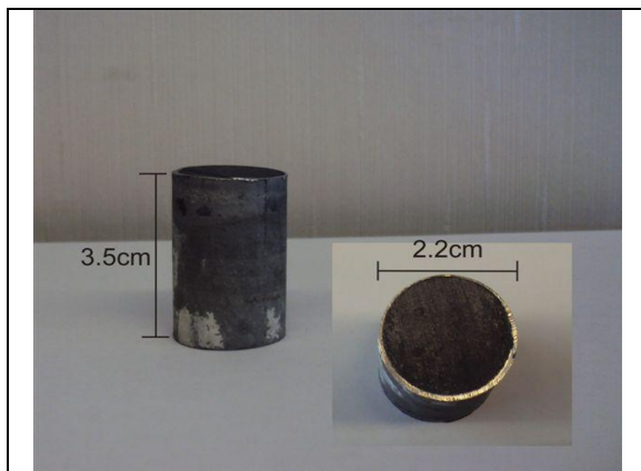
Figure 1. A356 Al-fly ash composite (C01)
