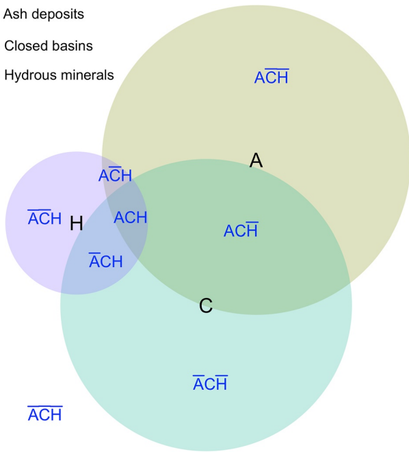
Figure 2. Venn diagram for the relations between binary patterns.
