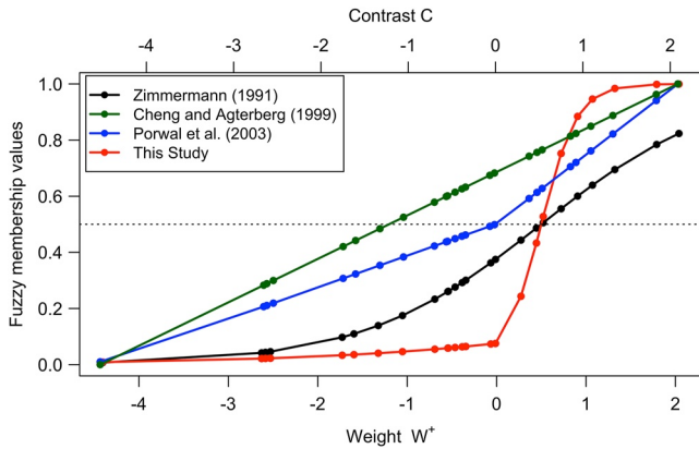
Figure 3. Calculation of fuzzy membership functions using different methods. The geology map (tn_geomp) was used as the example in this figure. The Weight W^+ x -axis refers to Method 1 (Zimmermann, 1991) and Method 4 developed in this study, while the Contrast C x -axis refers to Method 2 (Cheng & Agterberg, 1999) and Method 3 (Porwal et al., 2003).
