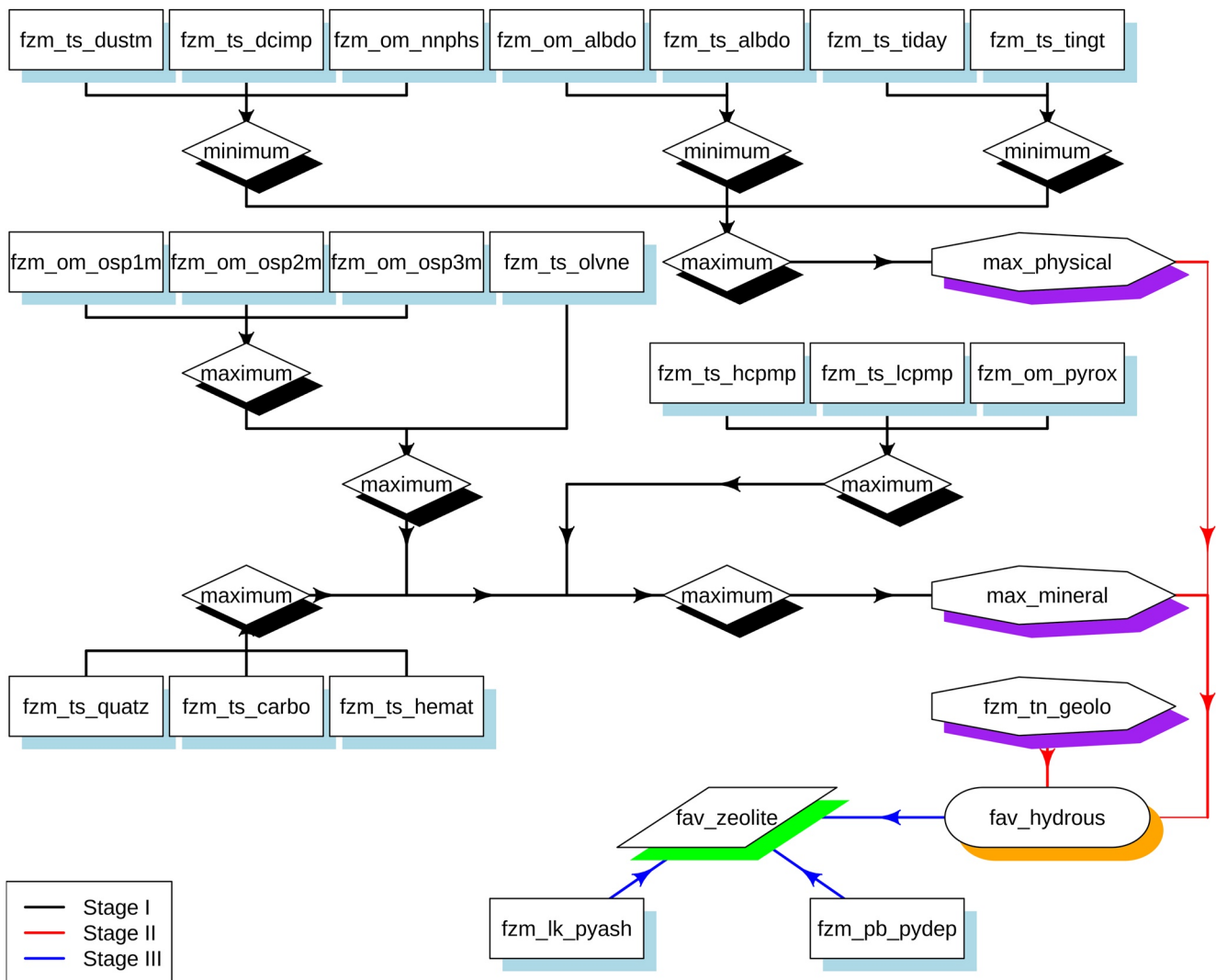
Figure 10. The fuzzy inference engine used to create the final map.
