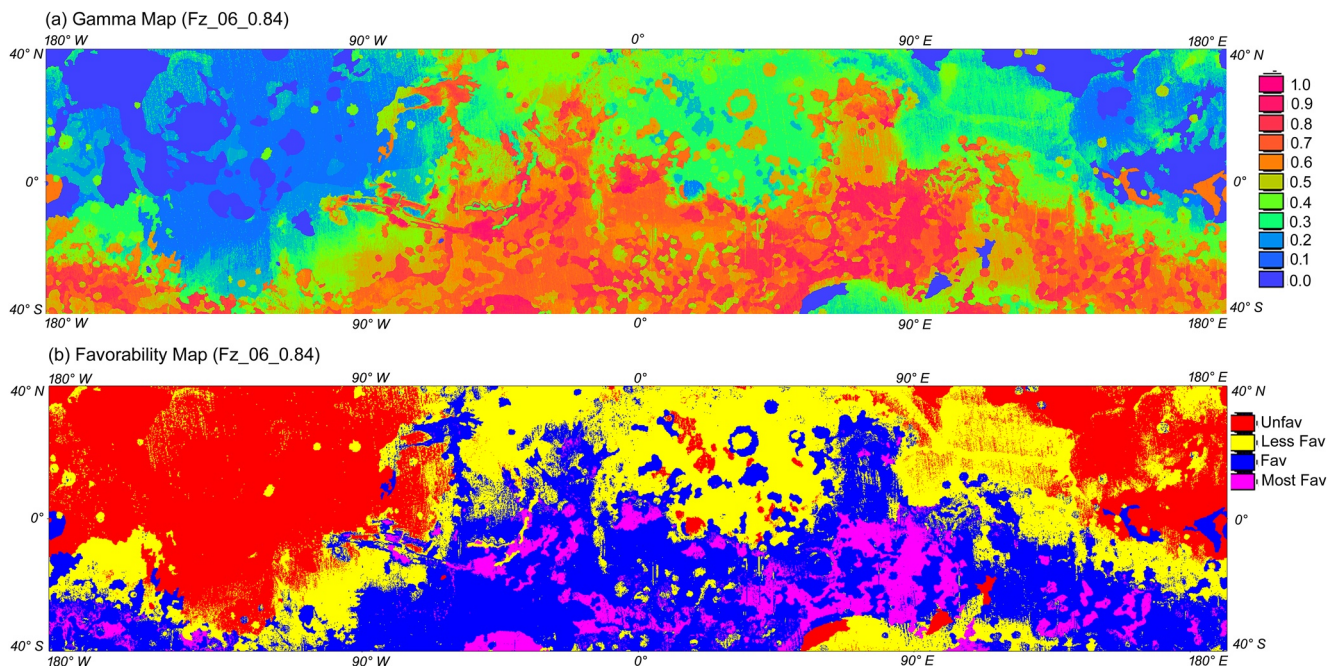
Figure 8. (a) Favorability map for hydrous minerals (Map Fz_06_0.84). The areas are ranked based on their fuzzy membership values. Fuzzy membership ranges from 0 to 1 (less favorable to highly favorable). (b) Favorability class map derived from map (a) showing the potential area for the hydrous minerals on Mars up to 40° latitude.
