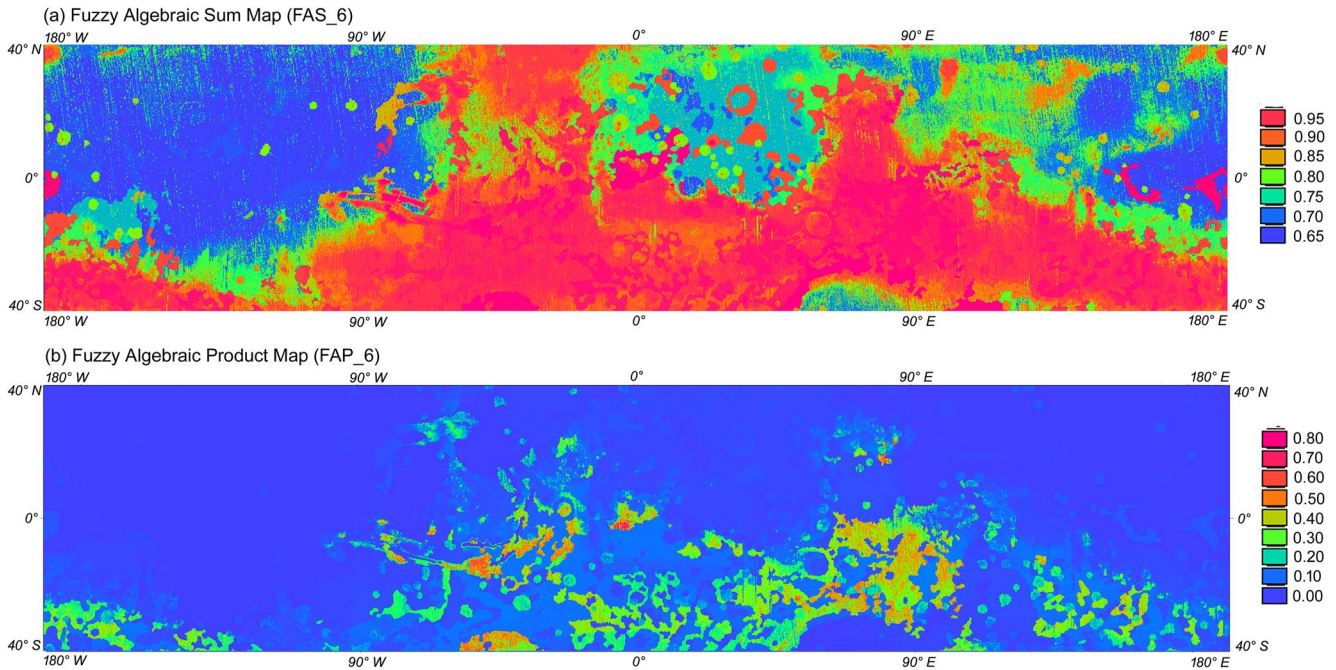
Figure 6. Fuzzy algebraic product (FAP) and fuzzy algebraic sum maps of map combination 6 (FAP_6 and FAS_6) listed in Table 4.
