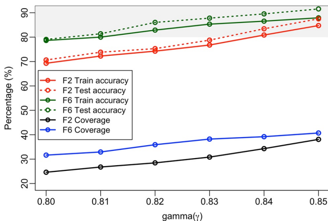
Figure 7. Percent accuracy and spatial coverage in each map combination (F2 and F6) against different gamma values.
