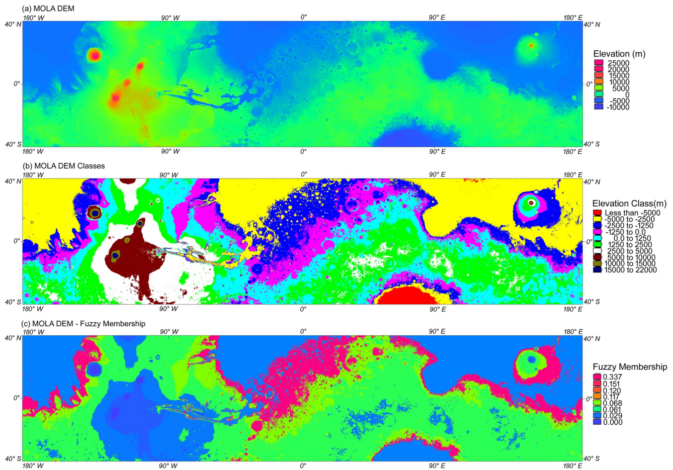
Figure 5. Fuzzification process showing (a) the original Mars Orbiter Laser Altimeter (MOLA) DEM, (b) classified MOLA DEM, and (c) a map after assigning the fuzzy membership values for each elevation class.
