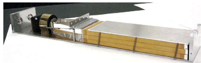
Fig. 7. Photo of one of the nine scintillator bricks. The three scintillator plates are individually wrapped and are 25 × 8 × 1 cm 3 (LWH). A single light guide channels the photons to the photomultiplier held in place with a simple collar.
