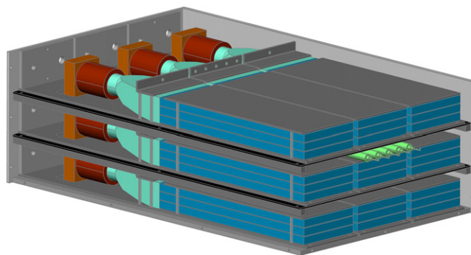
Fig. 6. Schematic drawing of the Neucal detector. Apart from the scintillator stacks (blue) described in the text, five 3 He tubes (green) are lodged at the centre of the detector. (For interpretation of the references to colour in this figure legend, the reader is referred to the web version of this article.)
