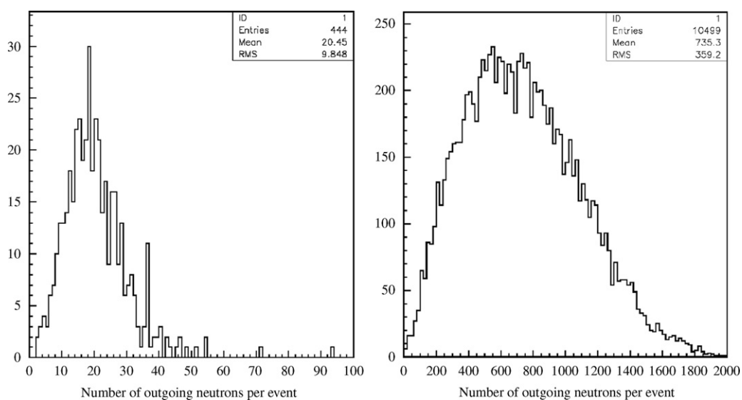
Fig. 2. Neutrons produced by 400 GeV electron (left) and 1 TeV proton (right) showering in the CALET calorimeters (FLUKA simulation).
